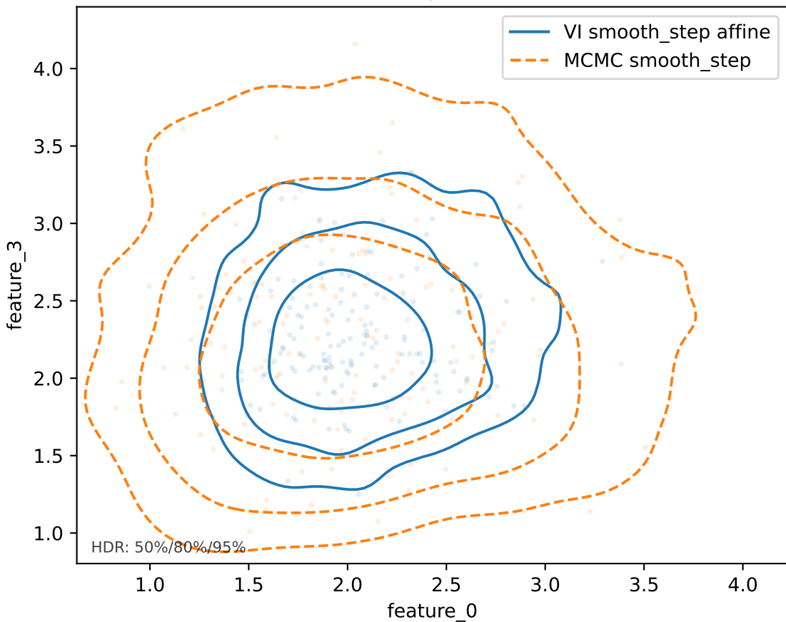
feature smooth step affine vs matched
