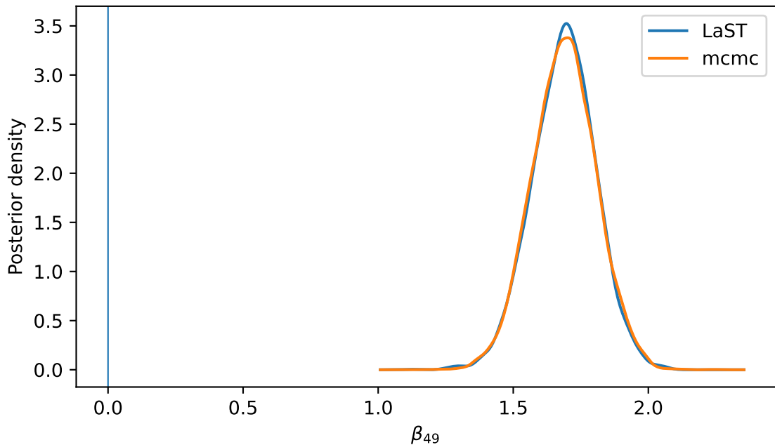
True-active marginal posterior recovery config E01, seed 400, \beta_{49}
