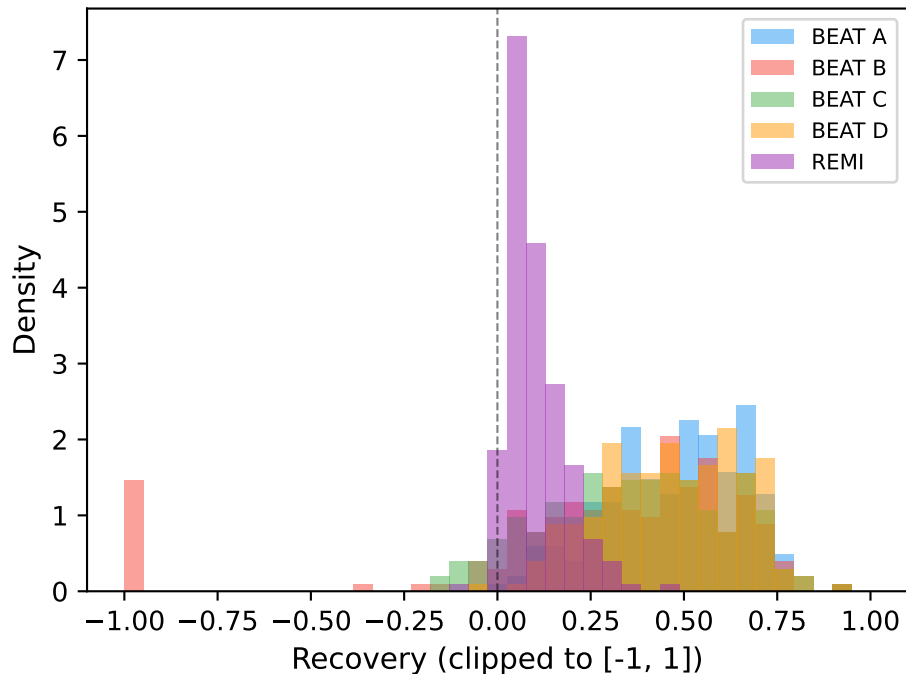
Recovery Distribution: All Schemes
