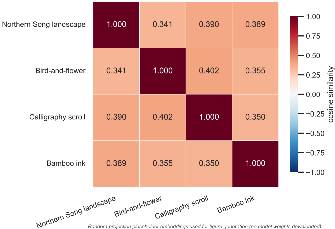
Cosine similarity of fused vectors z across 4 inputs
