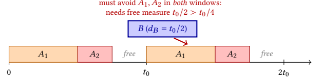
Figure 2: Proposition 2: at density 1, the per-window free set has measure t_0/4 , but B 's contiguous SP needs t_0/2 of it – in every window, under every placement.
