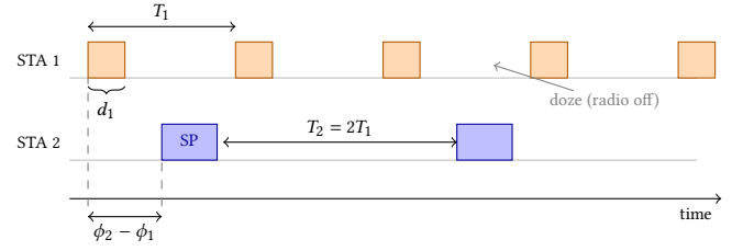
Figure 1: TWT wake schedules: station i wakes for d_i every T_i at offset \phi_i on a common (TSF-anchored) grid; the scheduler chooses the triples so that service periods are disjoint.
