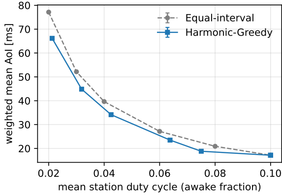
Figure 3: Weighted mean AoI vs. mean duty cycle across energy budgets ( 8\times weight skew, 10 stations, 5 seeds).
