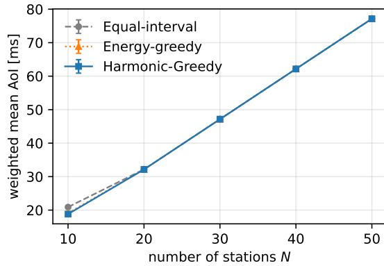
Figure 7: Scaling with the number of stations (8× weight skew, heterogeneous budgets, 3 seeds): all three schedulers track closely once the schedule is capacity-bound (energy floors pin the periods).
