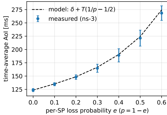
Figure 4: Single-station validation: measured time-average AoI (3 seeds, 95% CI) vs the renewal model, across per-SP loss probabilities ( T=100 ms, d=8 ms).
