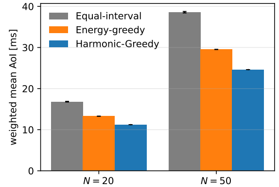
Figure 6: Heterogeneous modulation rates (HeMcs0/HeMcs7 alternating, 700-byte updates, 8\times weight skew, 3 seeds): the gain decomposes into period diversity (energy-greedy over equal-interval) and AoI-weighting (HARMONIC-GREEDY over energy-greedy); 36% total at N=50 .
