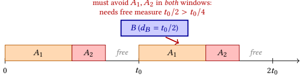
Figure 2: Proposition ??: at density 1, the per-window free set has measure t_0/4 , but B 's contiguous SP needs t_0/2 of it – in every window, under every placement.
