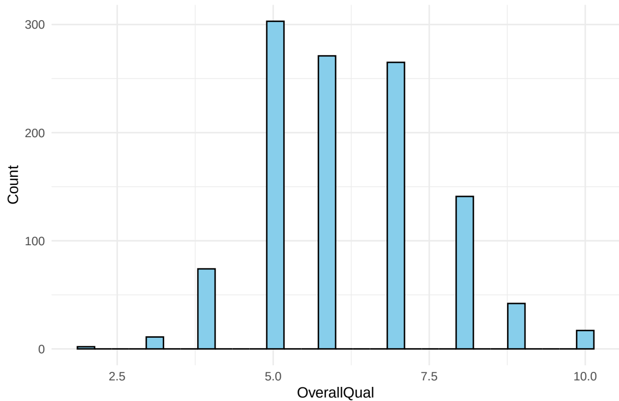
Histogram of OverallQual
