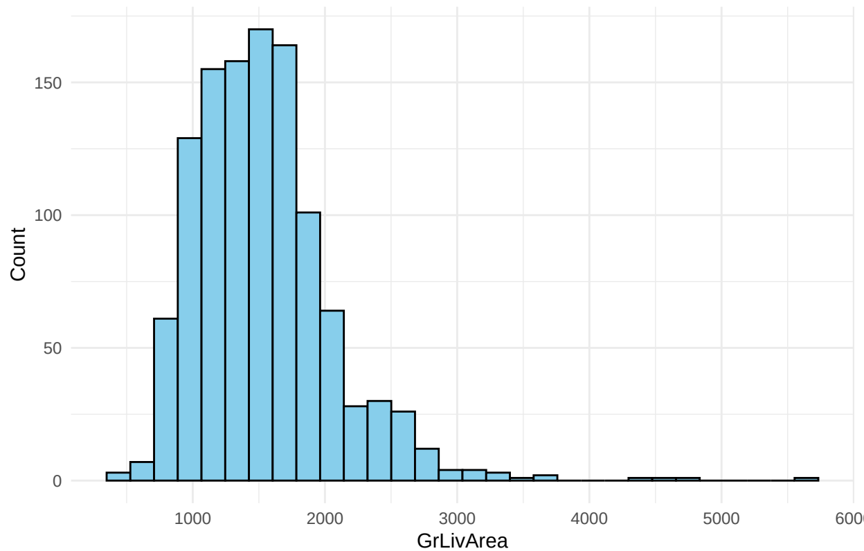
Histogram of GrLivArea
