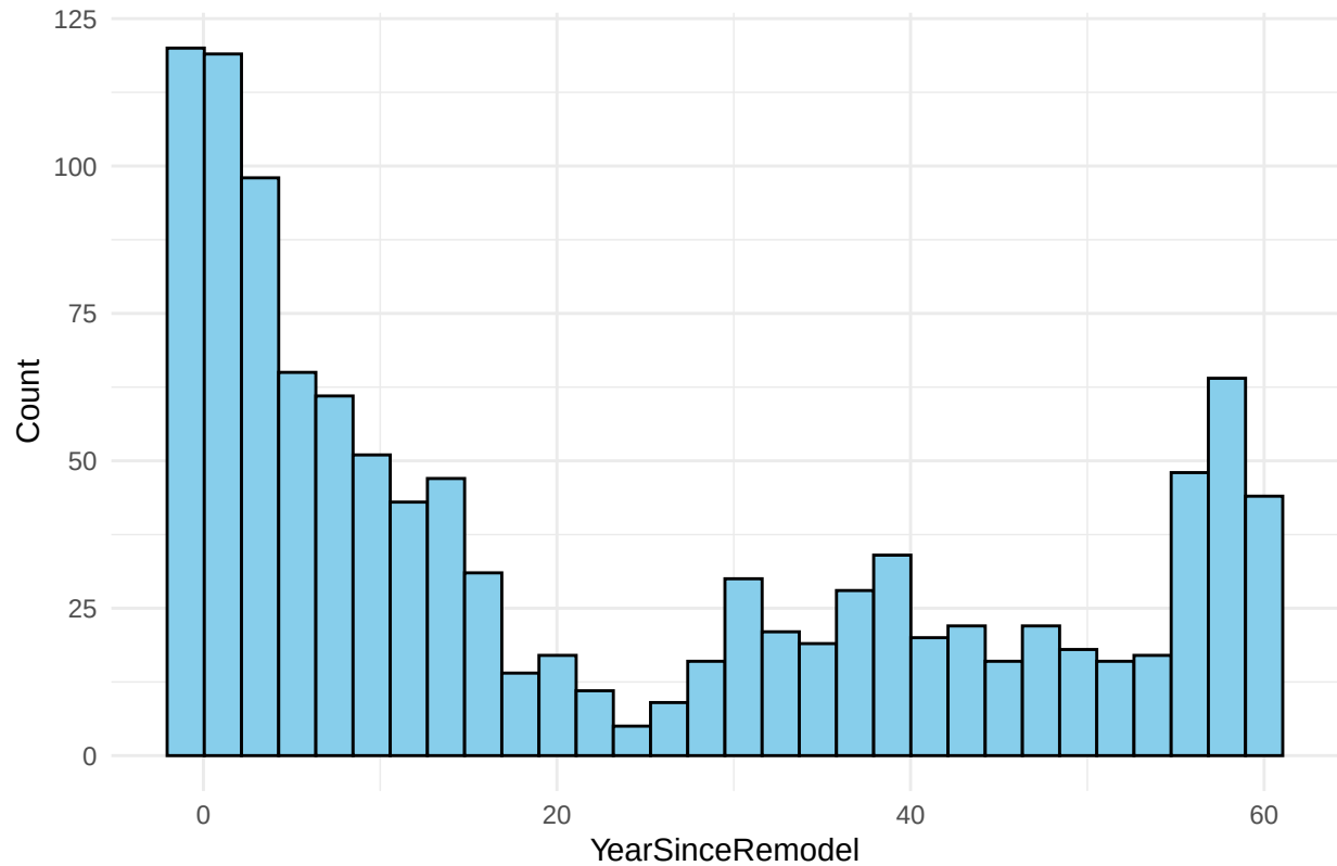
Histogram of YearSinceRemodel
