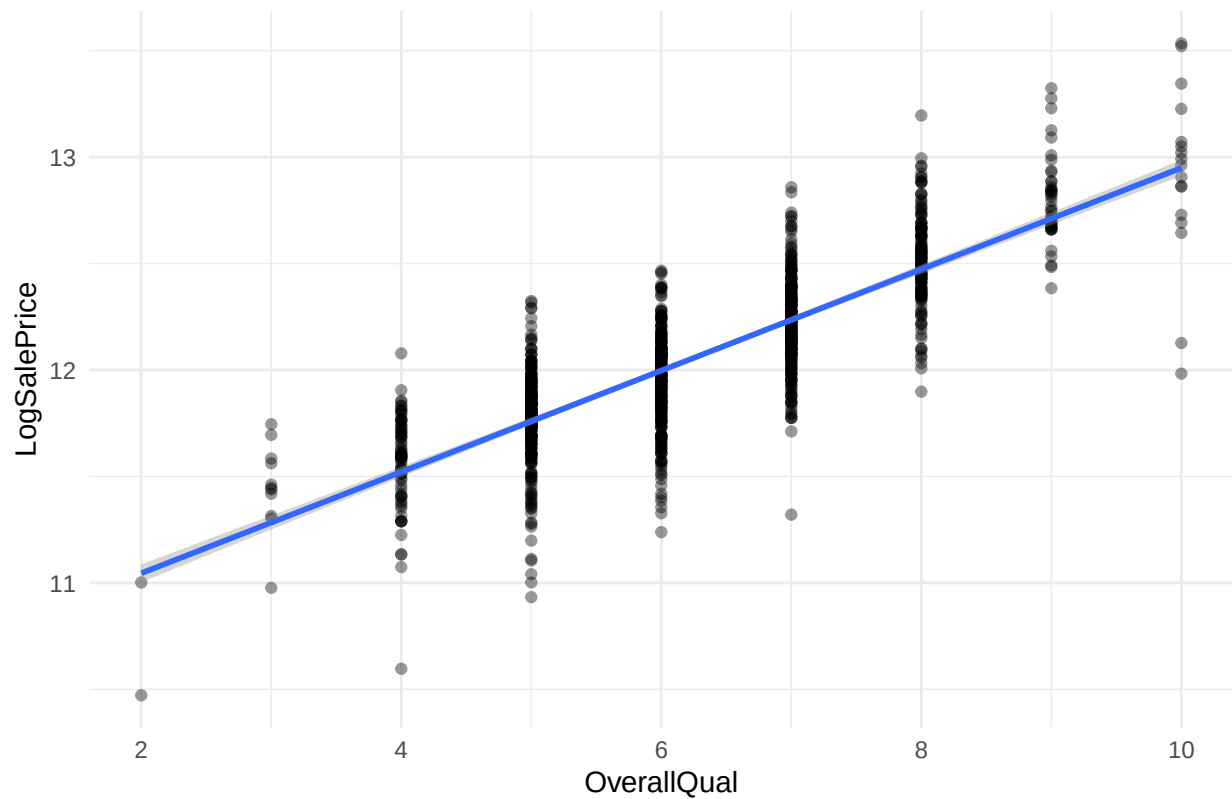
LogSalePrice vs OverallQual
