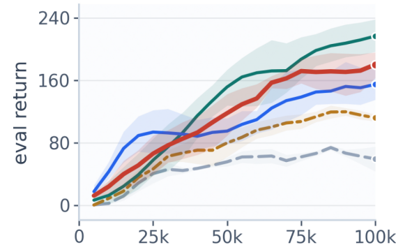
Cheetah Run
