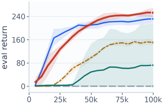
Finger Spin
