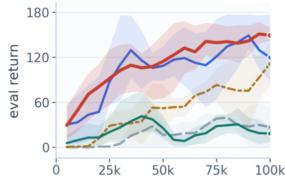
Reacher Easy
