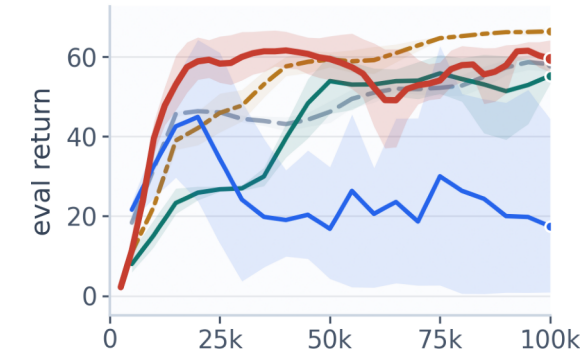
Cartpole Swingup
