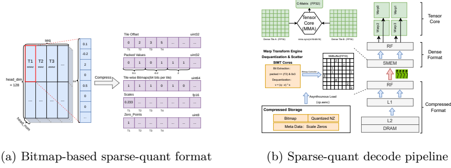
Fig. 4. Overview of the sparse-quant format and attention kernel. The left panel shows the bitmap-based sparse-quant storage format. The right panel shows the decode pipeline that loads compressed tiles, performs unpacking and dequantization, reconstructs dense shared-memory tiles, and invokes Tensor Core matrix-vector computation.
