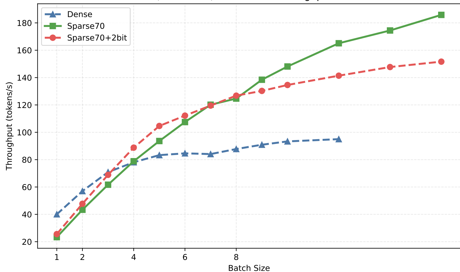
Llama-3 8B (4096→256): End-to-End Throughput vs Batch Size
