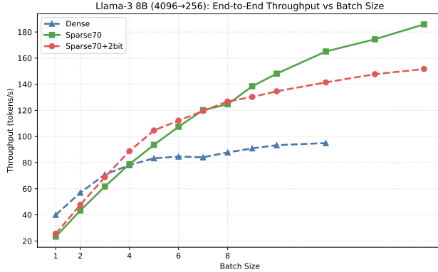
Fig. 5. End-to-end decoding throughput on Meta-Llama-3-8B-Instruct with 4096 input tokens and 256 output tokens. The full sparse-quant path provides its most visible advantage in the small-to-medium batch regime.
