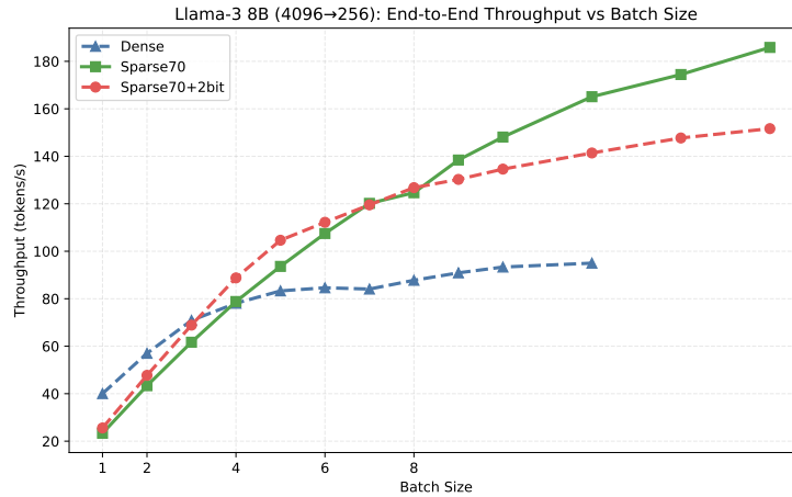
Fig. 5. End-to-end decoding throughput on Meta-Llama-3-8B [7] with 4096 input tokens and 256 output tokens. The full sparse-quant path provides the clearest advantage in the small-to-medium batch regime.
