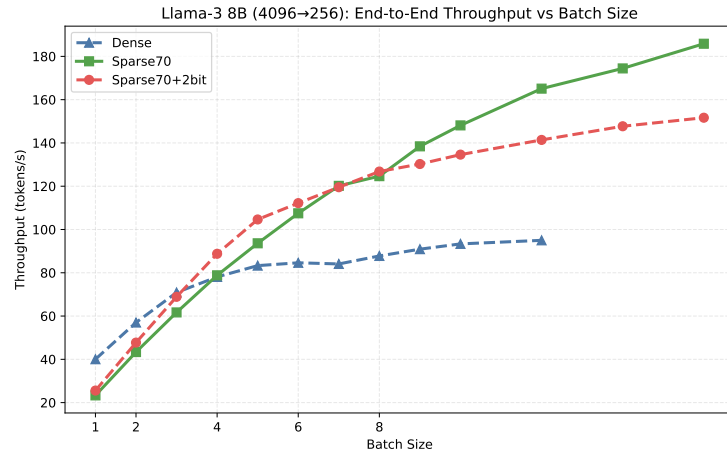
Fig. 5. End-to-end decoding throughput on Meta-Llama-3-8B-Instruct [7] with 4096 input tokens and 256 output tokens. The full sparse-quant path provides the clearest advantage in the small-to-medium batch regime.
