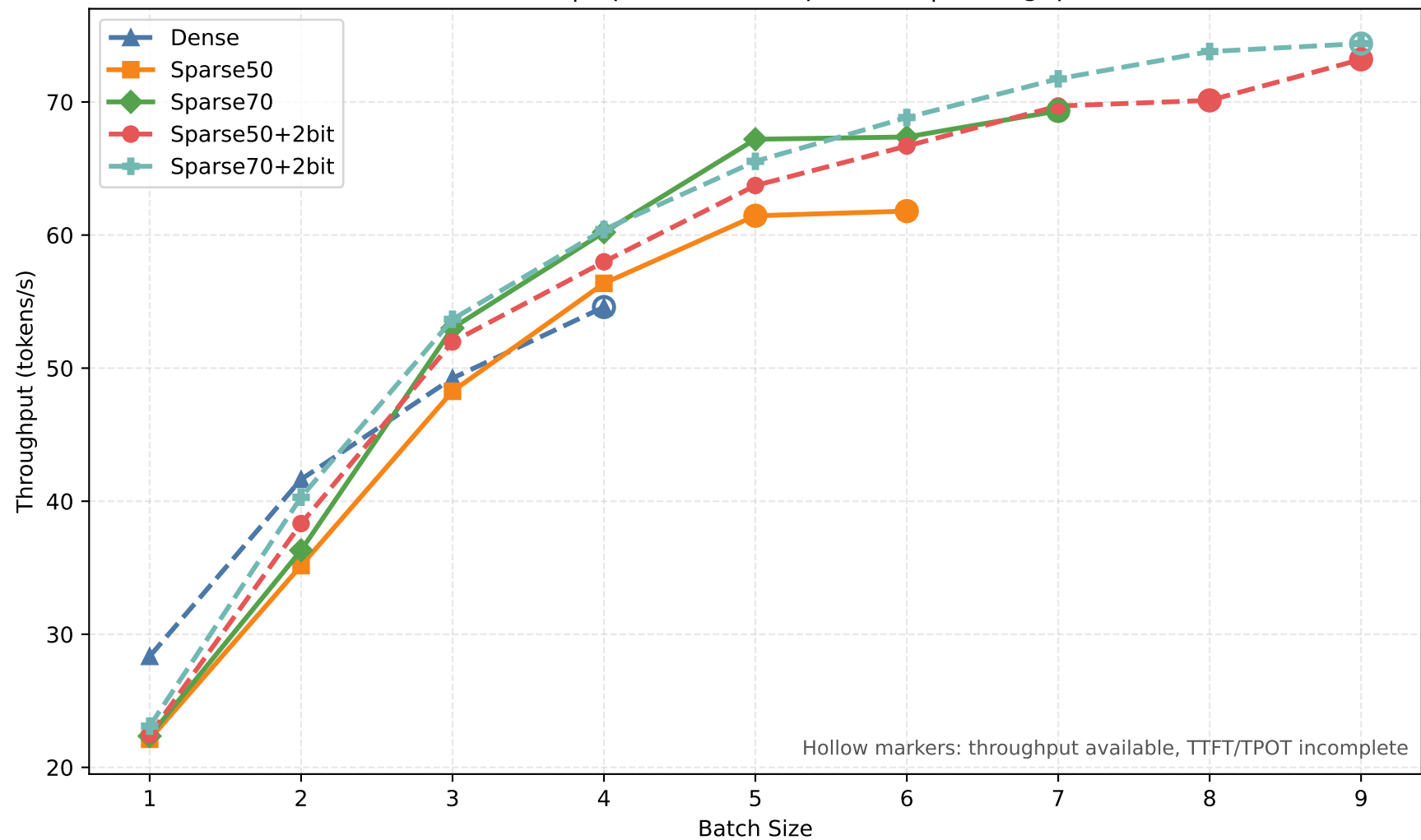
Meta-Llama-3-8B-Instruct | input=4096, output=256 | Throughput vs Batch Size
