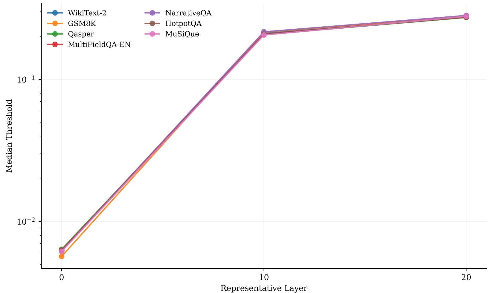
Median Threshold Profiles Across Datasets
