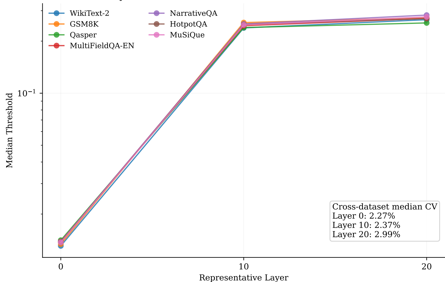
Layer-Wise Median Threshold Profiles Across Datasets
