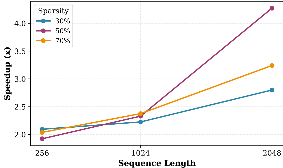
(b) Speedup vs. Scale
