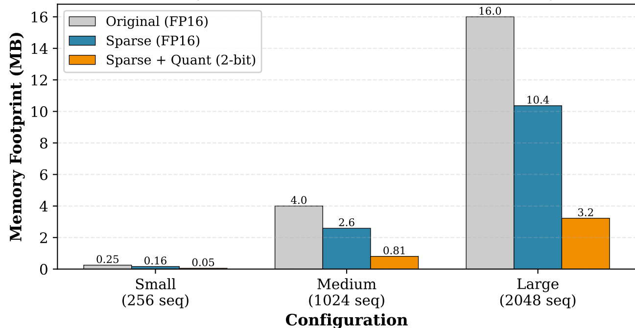
Memory Footprint Comparison (50% Sparsity)
