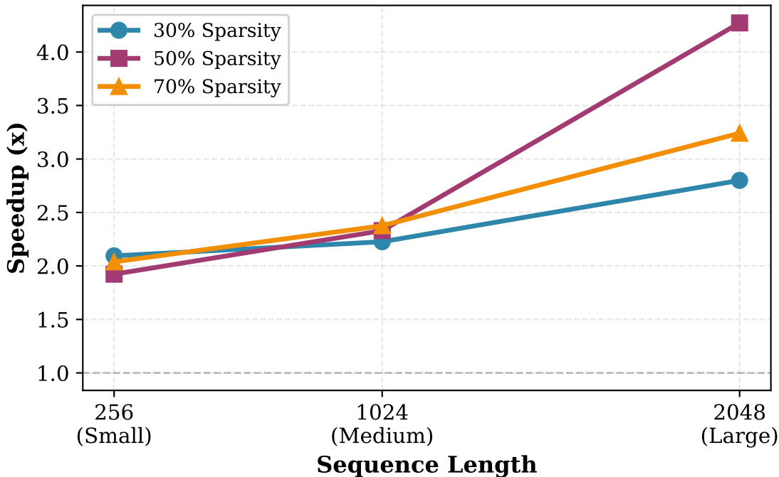
Compression Speedup vs. Sequence Length
