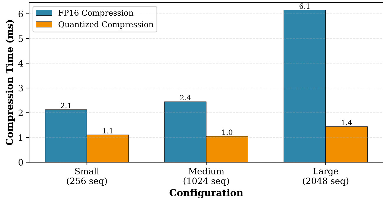
Compression Time Comparison (50% Sparsity, median)
