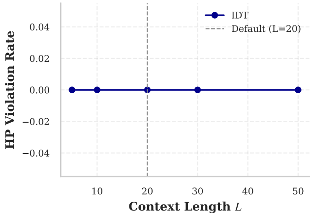
(b) Context Length vs HP Violation
