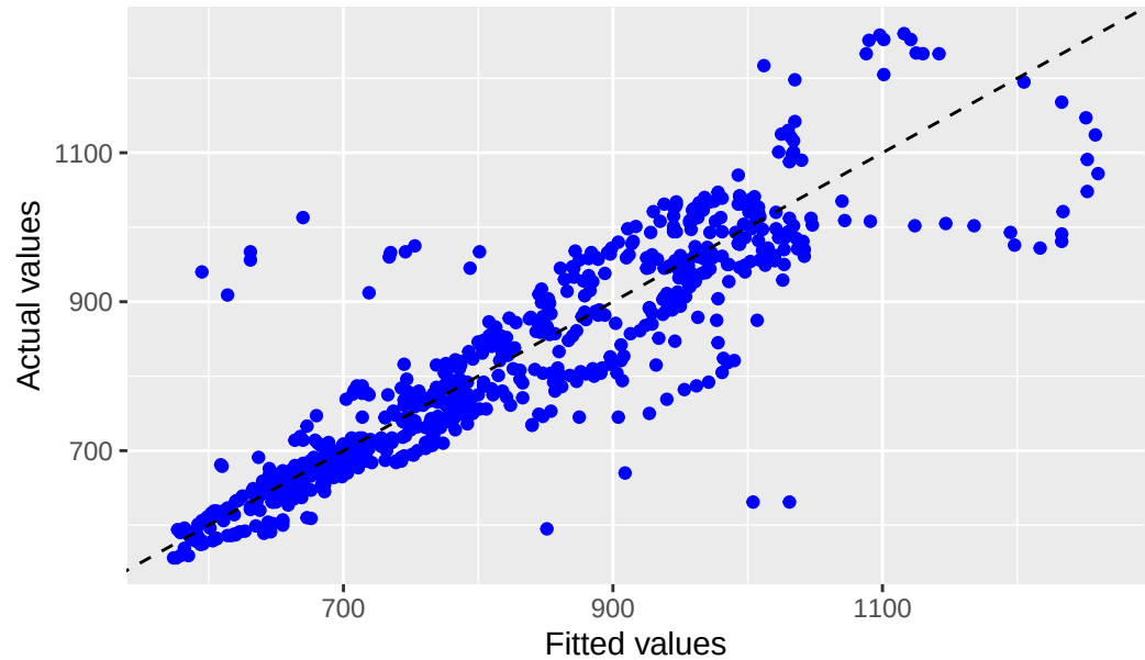
Actual vs. Fitted Values: Seasonal Naive Model
