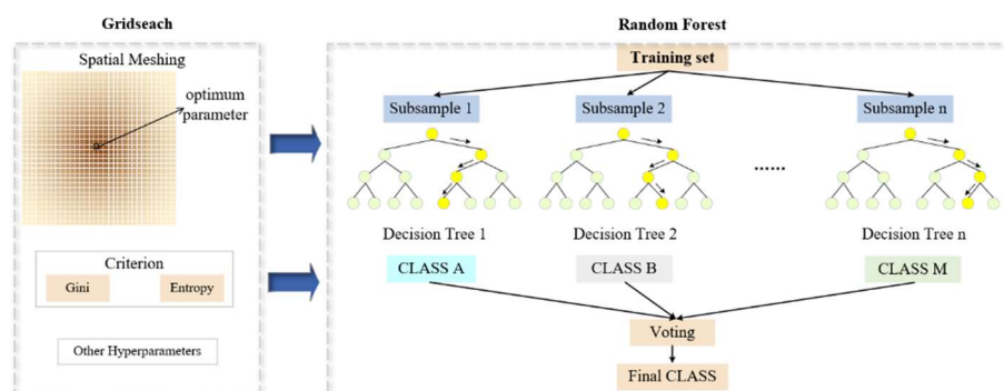
Figure 4 GSRF Algorithm Flow Diagram
