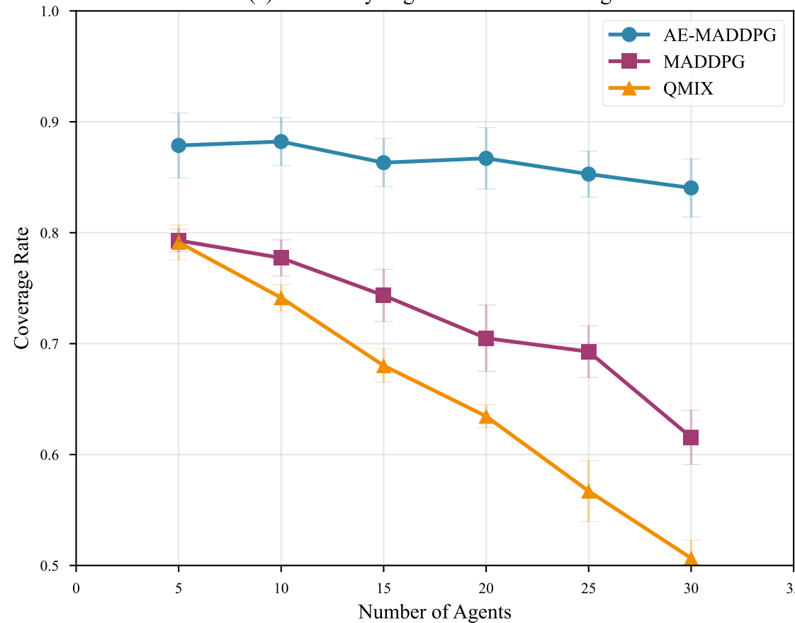
(a) Scalability: Agent Count vs Coverage
