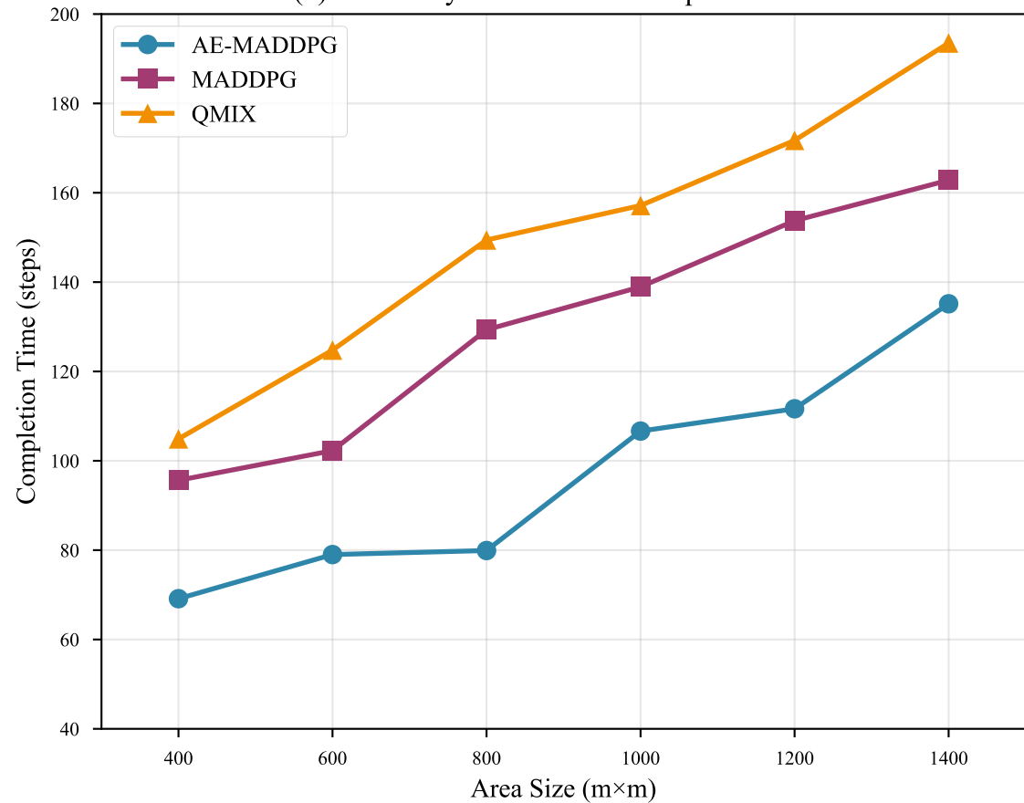
(b) Scalability: Area Size vs Completion Time
