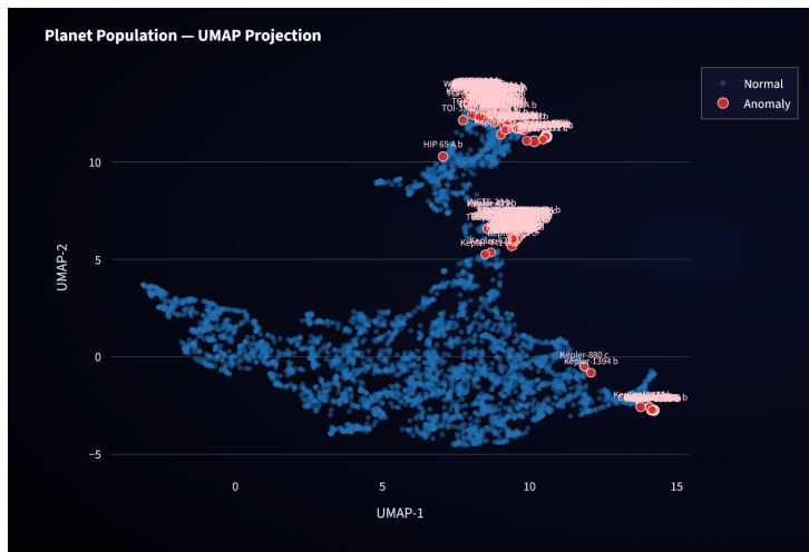
Figure 9: UMAP 2D projection of catalog planets, with anomaly candidates highlighted by the Isolation Forest-based detection module.
