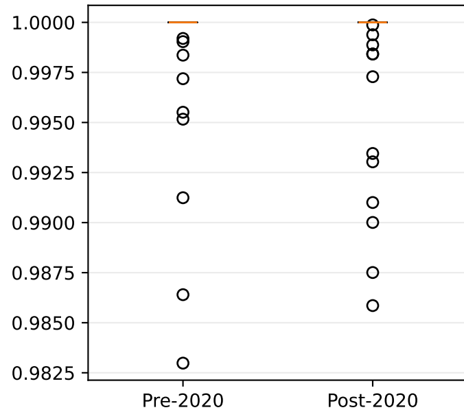
Median Hurst Exponent
