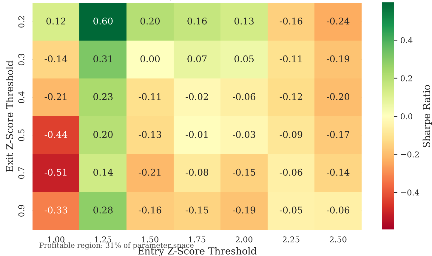
Parameter Sensitivity: BAC/PNC OOS Sharpe Ratio
