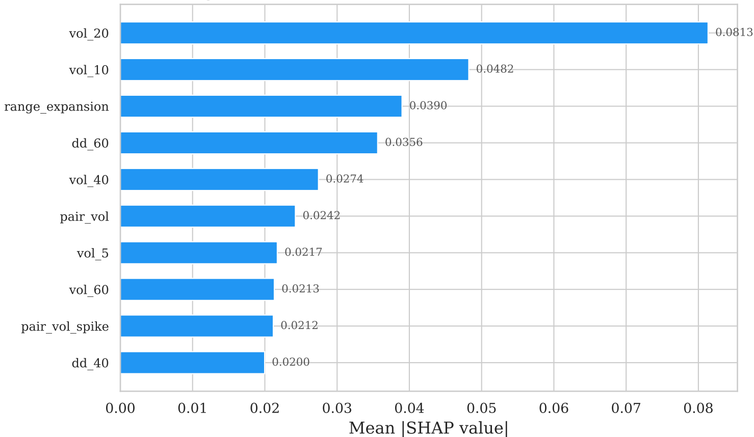
RF Regime Classifier: Top-10 Feature Importance (SHAP)
