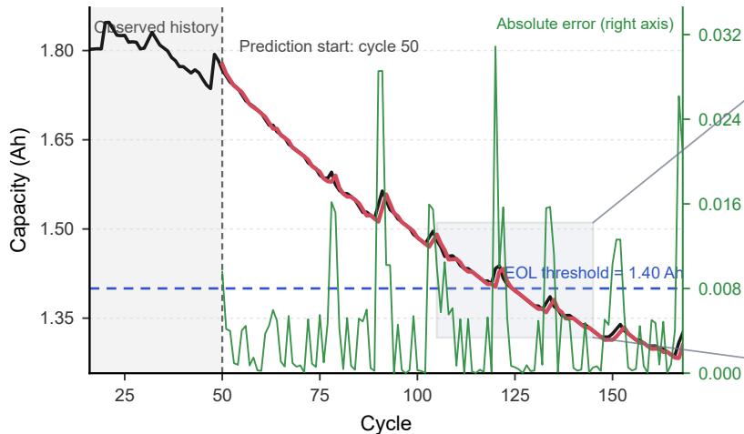
Full trajectory (B0005)
