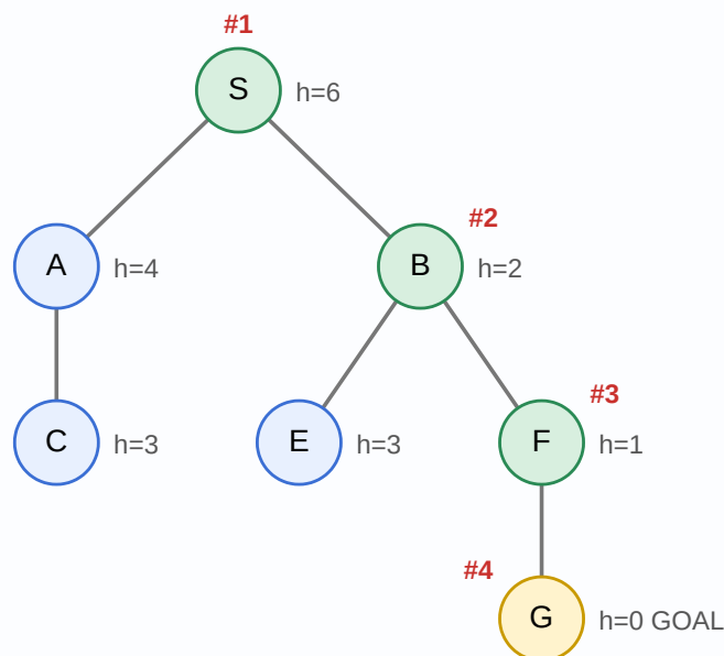
Figure 3d. Greedy best-first: always expand the child with the smallest h \rightarrow path S \rightarrow B \rightarrow F \rightarrow G (green). Fast, but not guaranteed optimal
