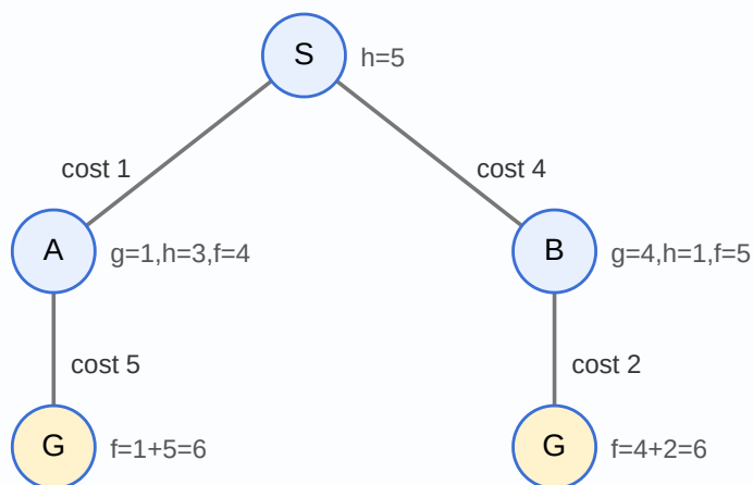
Figure 3e. A* ( f = g + h ) expands A ( f=4 ) before B ( f=5 ); Greedy ( f = h ) would pick B first ( h=1 )
