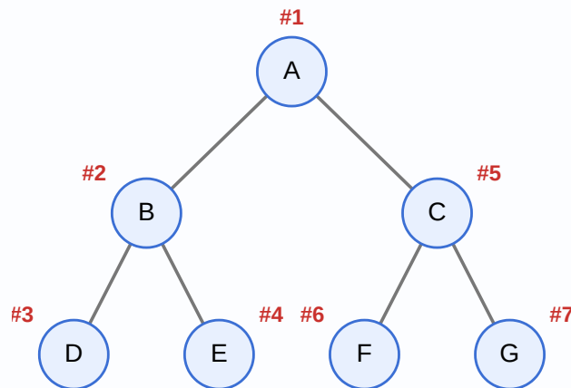
Figure 3b. Depth-First Search – go deep, then backtrack (LIFO stack): A B D E C F G
