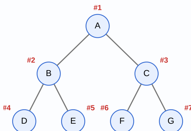
Figure 3a. Breadth-First Search – visit level by level (FIFO queue): A B C D E F G
