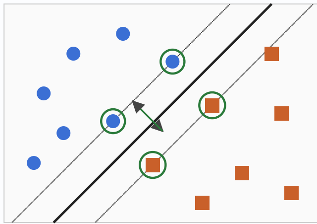
Figure 13. SVM: the widest 'street' between the two classes; only the support vectors fix its position
