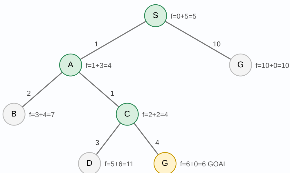
Figure 3f. A* search tree: at each step expand the node with the smallest f ; green path S → A → C → G ( f = 6 )
