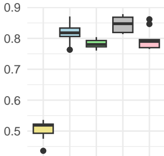
MRR
