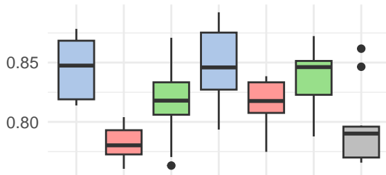
MRR
