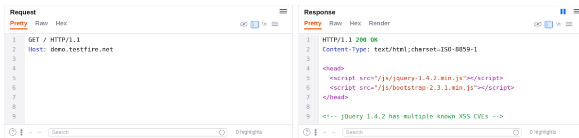
Figure 7. The page source references jQuery 1.4.2, a version affected by multiple known XSS vulnerabilities.
