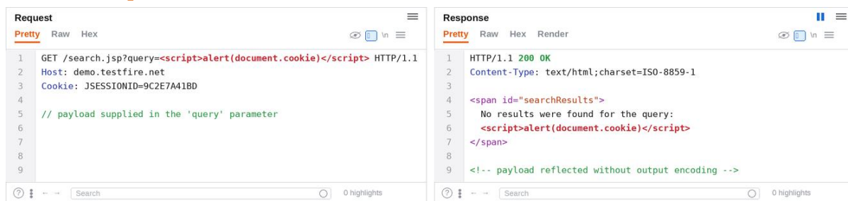
Figure 3. Burp Repeater — the script payload is reflected unencoded and executes in the browser, leaking document.cookie .
