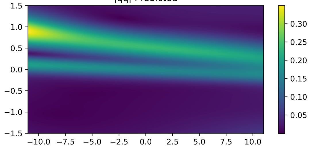
|qq| Predicted
