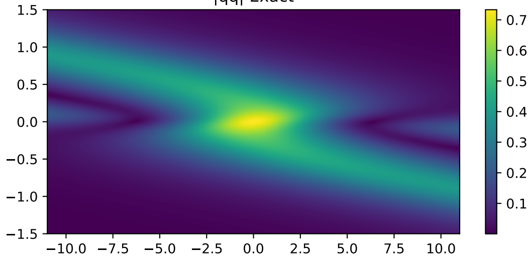
|qq| Exact
