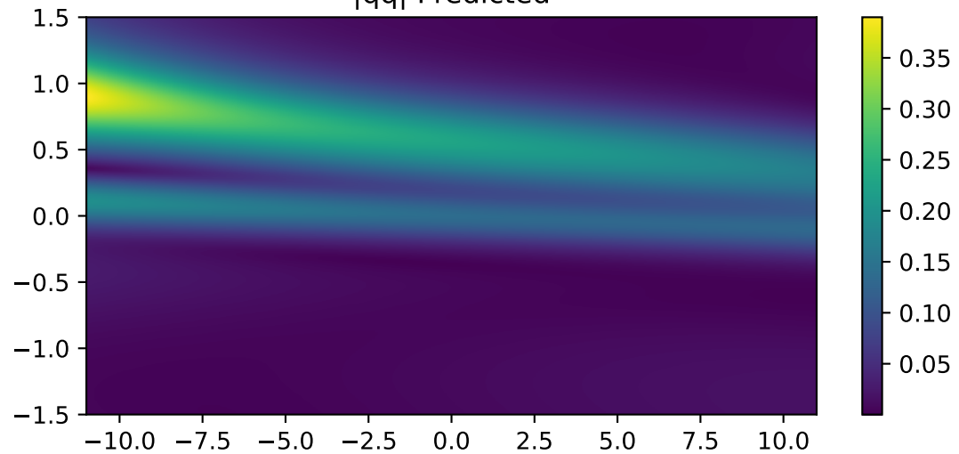
|qq| Predicted
