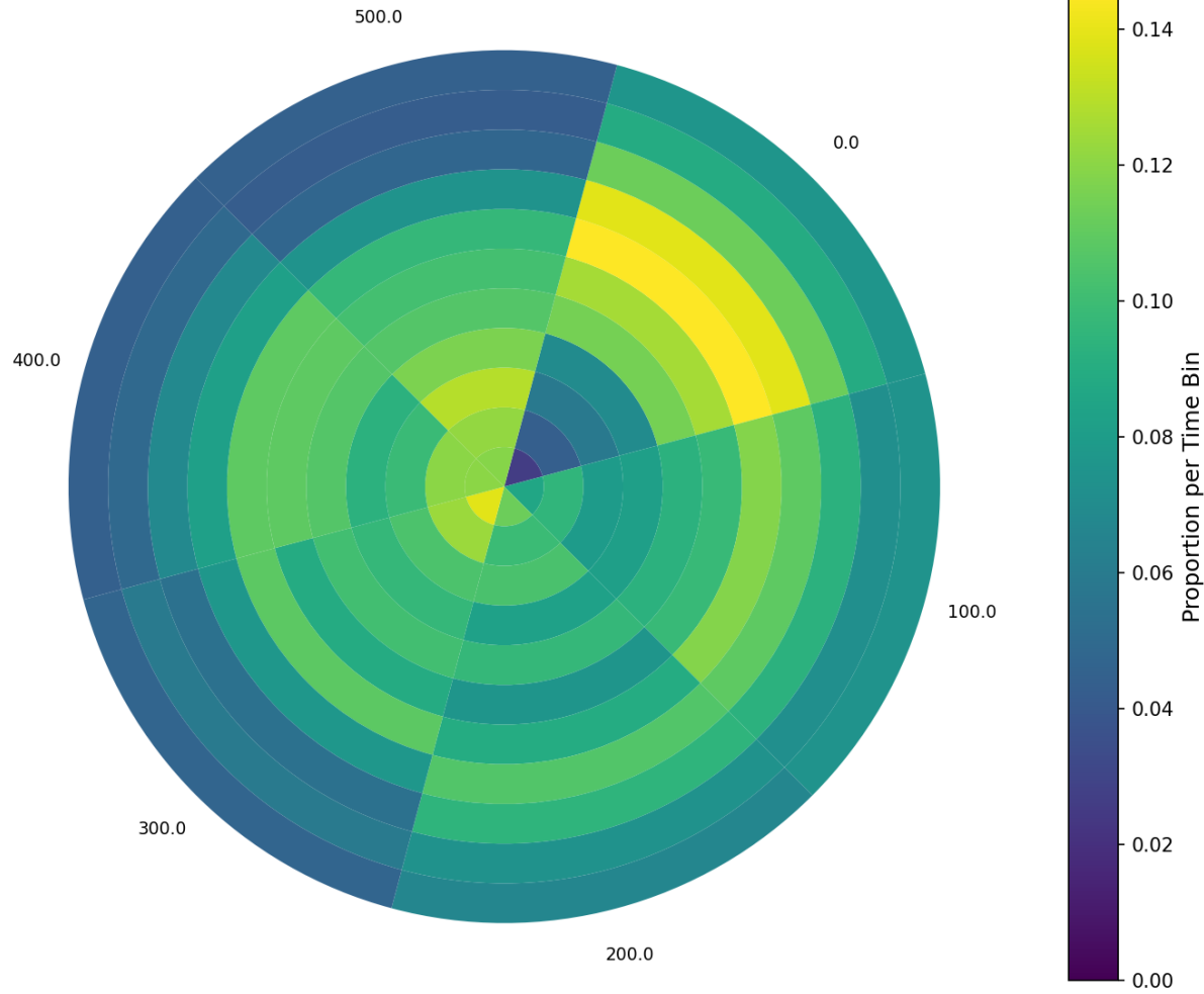
Radial Sholl (Per-Bin Normalized) – Condition: EA TNTixMPN Fed Group 10-5
