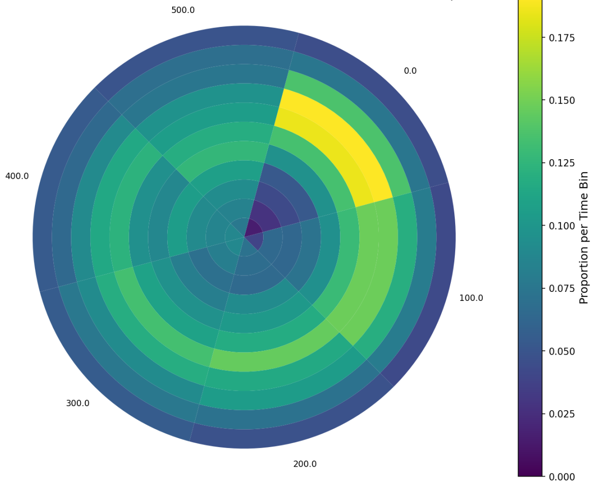
Radial Sholl (Per-Bin Normalized) - Condition: EA TNTexMPN Fed Group 10-5
