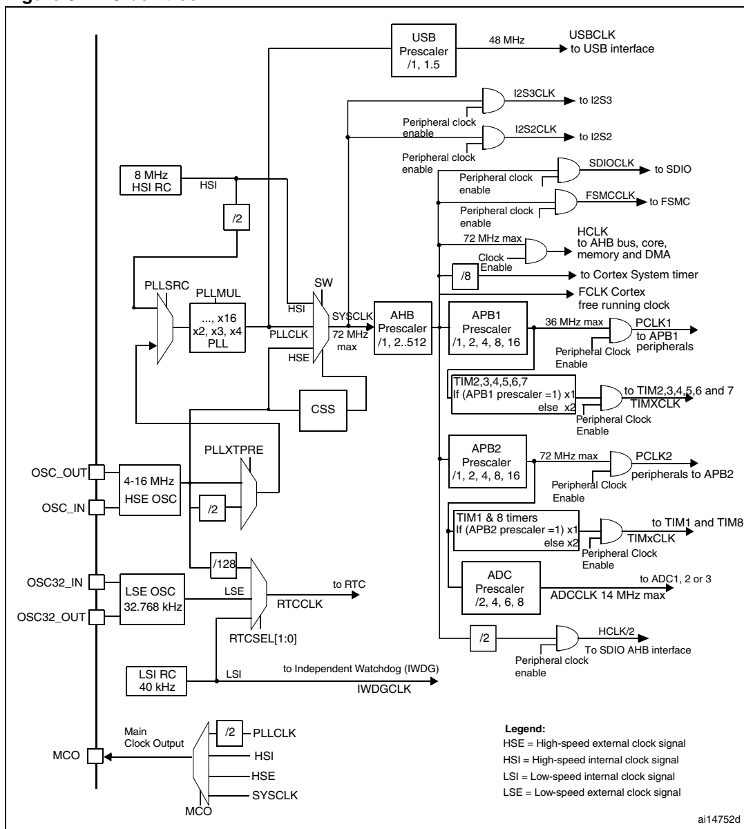
Figure 8. Clock tree
