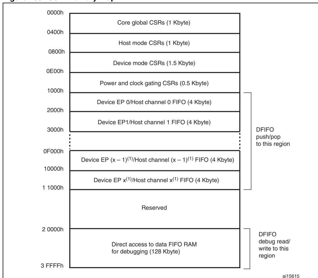
Figure 269. CSR memory map
