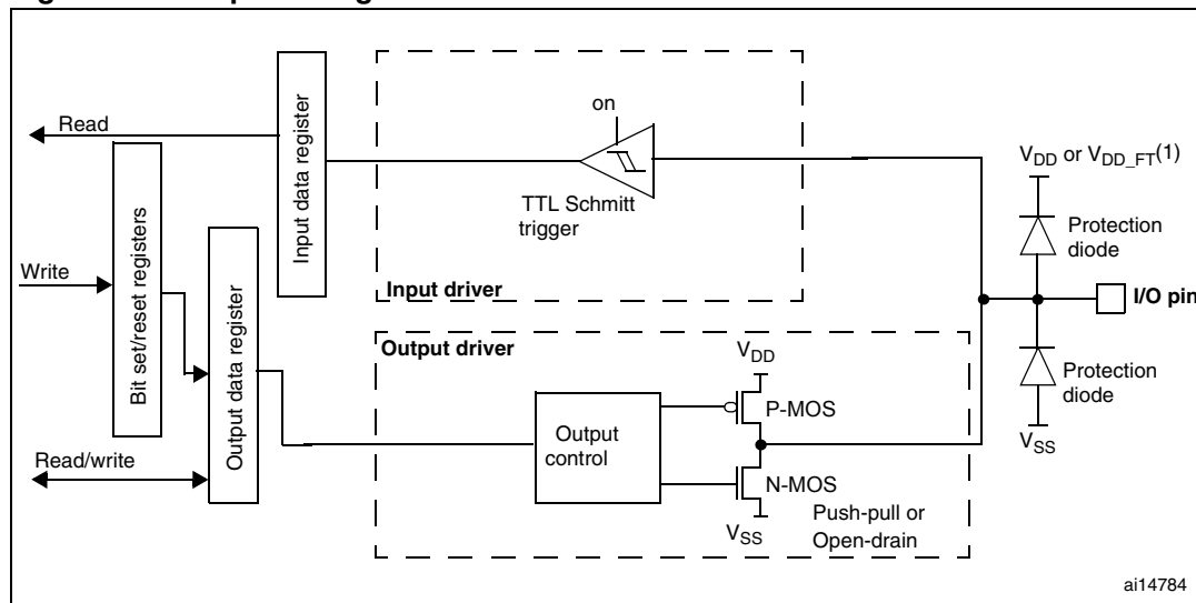
Figure 16. Output configuration
