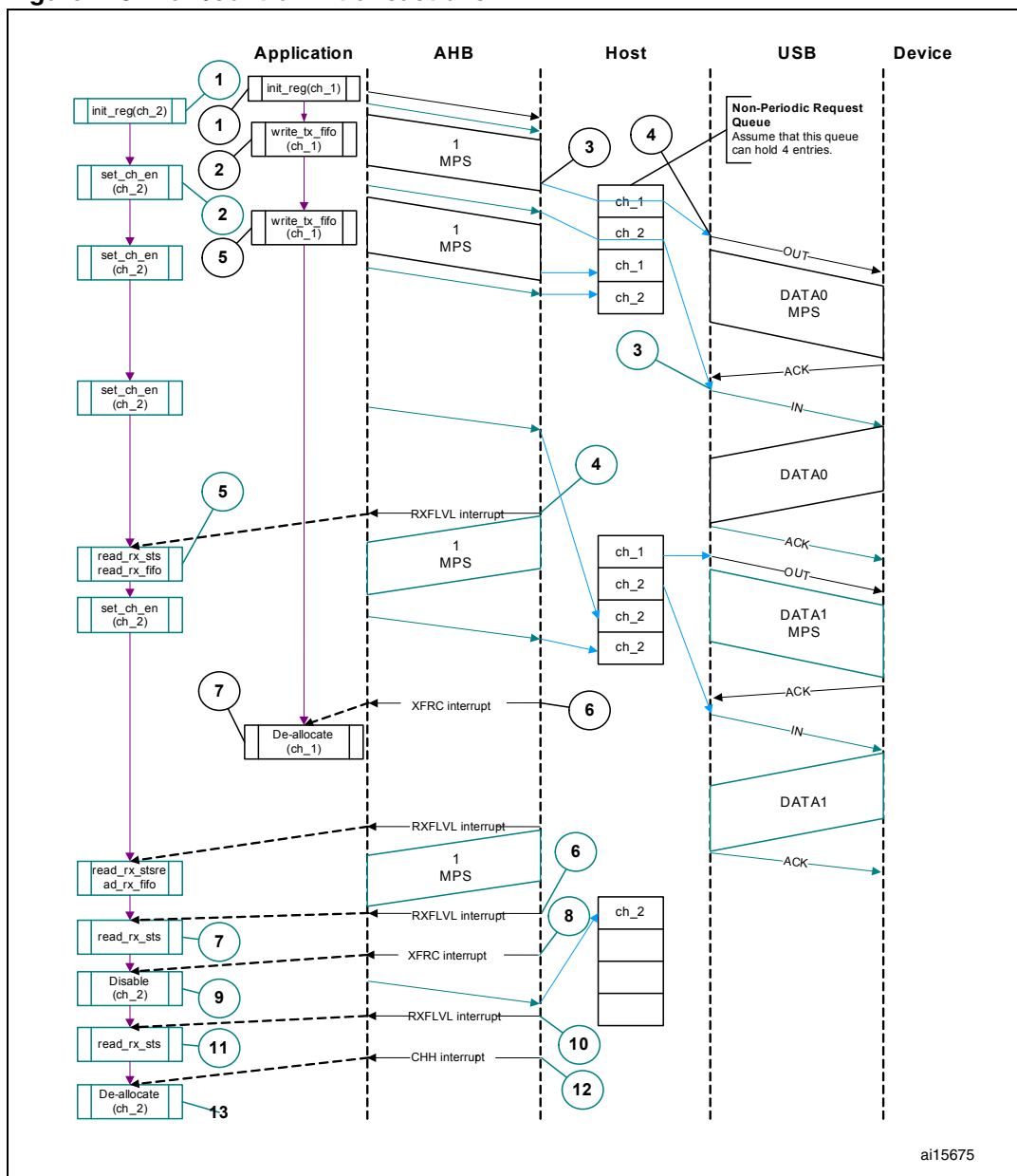
Figure 273. Bulk/control IN transactions
