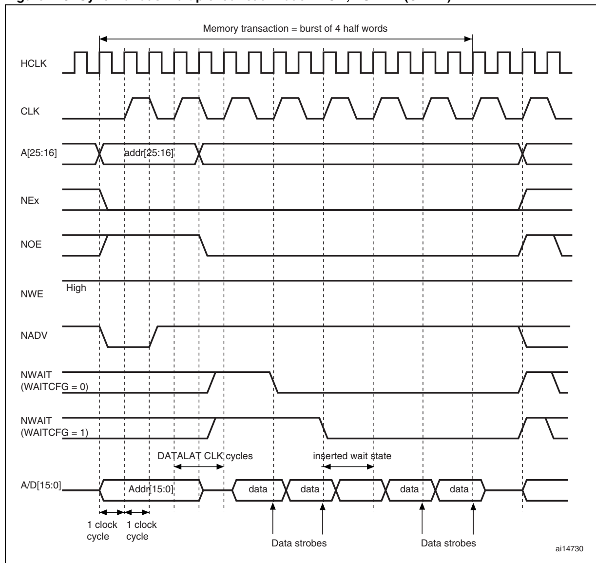
Figure 173. Synchronous multiplexed read mode - NOR, PSRAM (CRAM)
