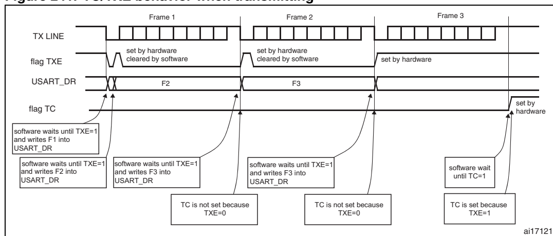
Figure 241. TC/TXE behavior when transmitting
