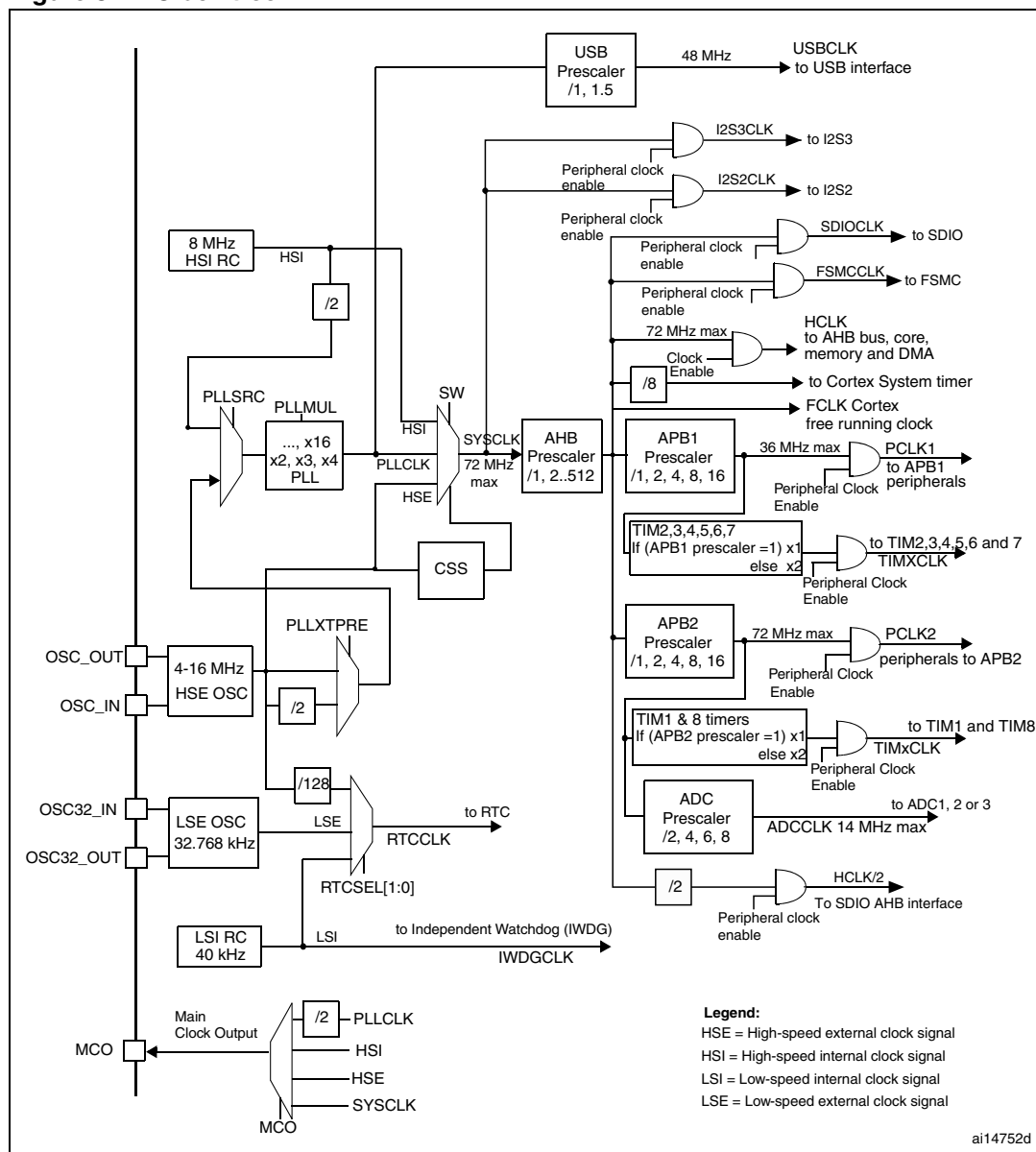
Figure 8. Clock tree
