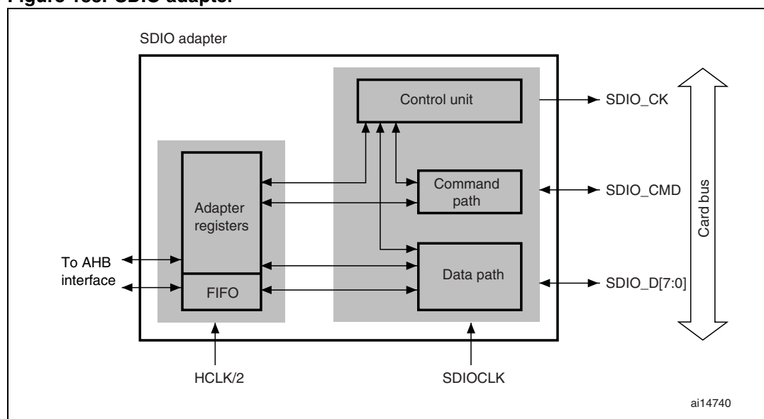
Figure 183. SDIO adapter
