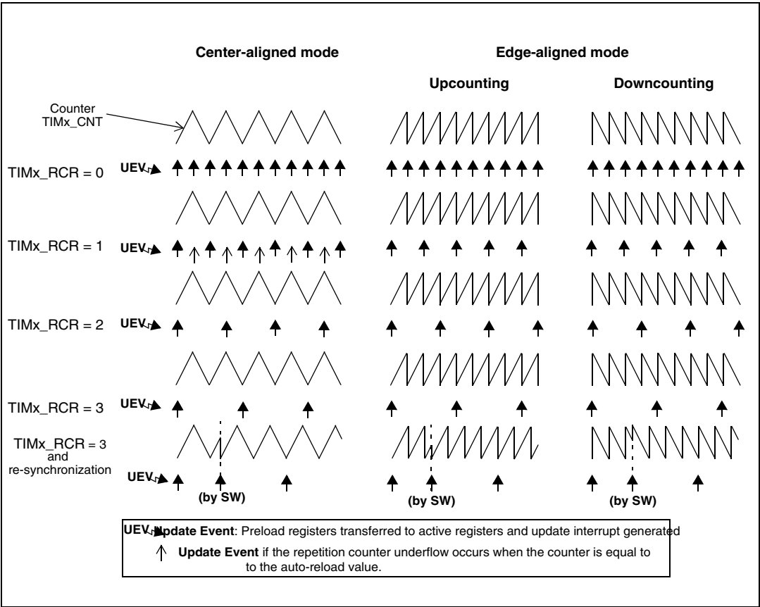
Figure 71. Update rate examples depending on mode and TIMx_RCR register settings
