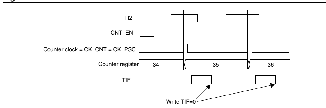
Figure 74. Control circuit in external clock mode 1
