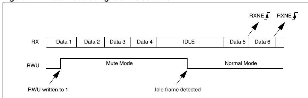
Figure 244. Mute mode using Idle line detection
