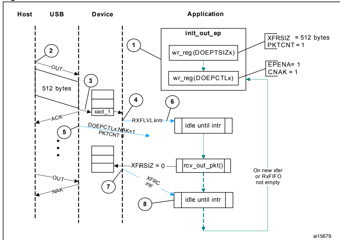
Figure 278. Slave mode bulk OUT transaction
