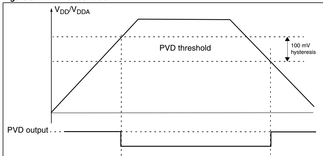
Figure 6. PVD thresholds
