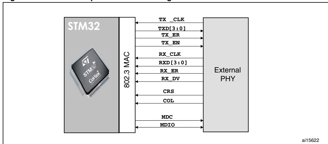
Figure 288. Media independent interface signals
