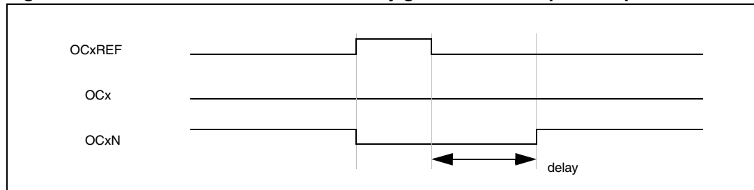
Figure 87. Dead-time waveforms with delay greater than the positive pulse.
