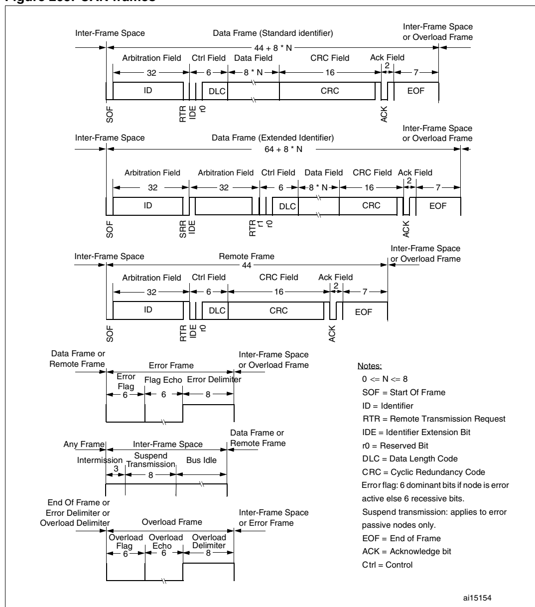
Figure 205. CAN frames
