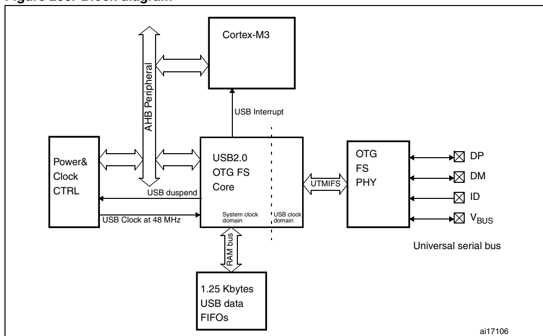
Figure 260. Block diagram
