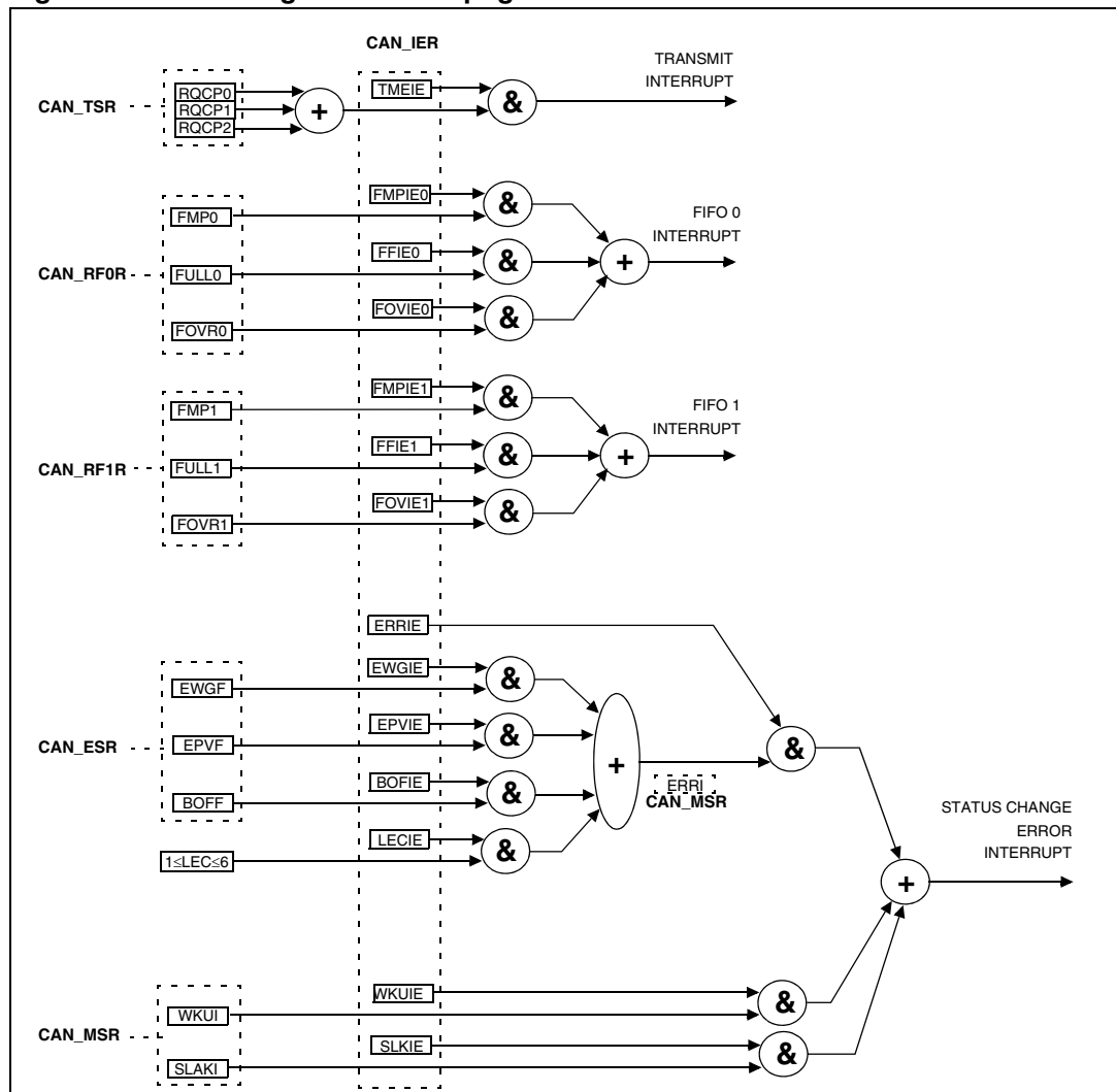
Figure 206. Event flags and interrupt generation
