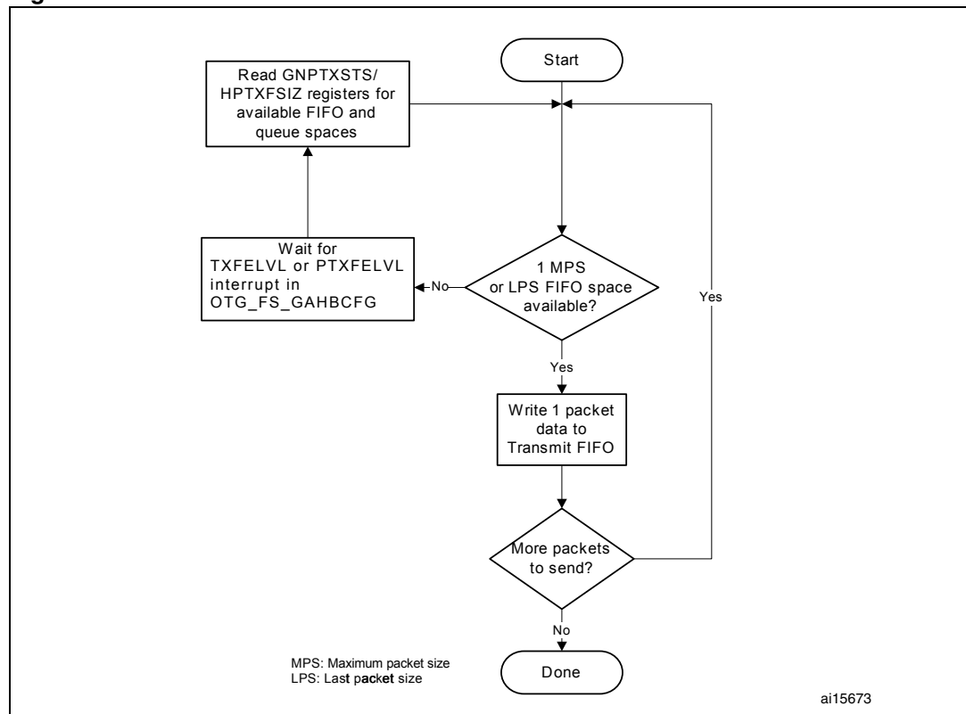
Figure 270. Transmit FIFO write task
