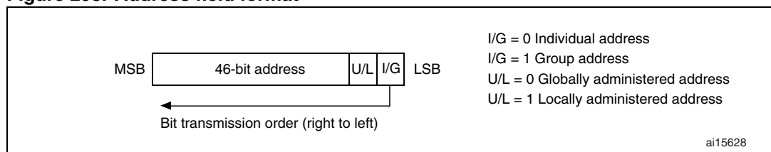
Figure 293. Address field format
