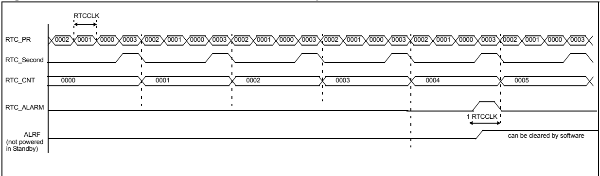
Figure 156. RTC second and alarm waveform example with PR=0003, ALARM=00004
