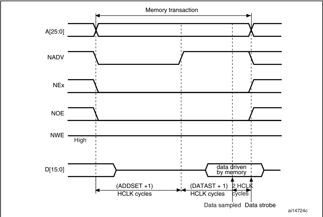
Figure 165. Mode2/B read accesses
