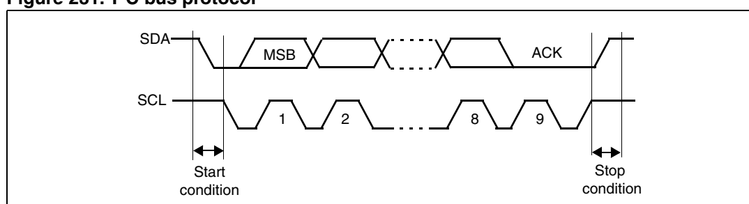
Figure 231. I 2 C bus protocol
