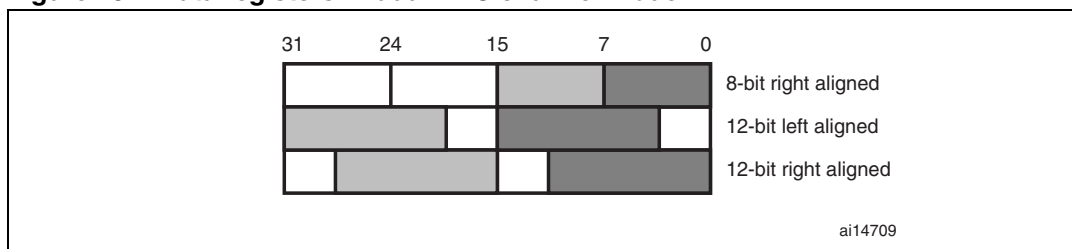
Figure 45. Data registers in dual DAC channel mode
