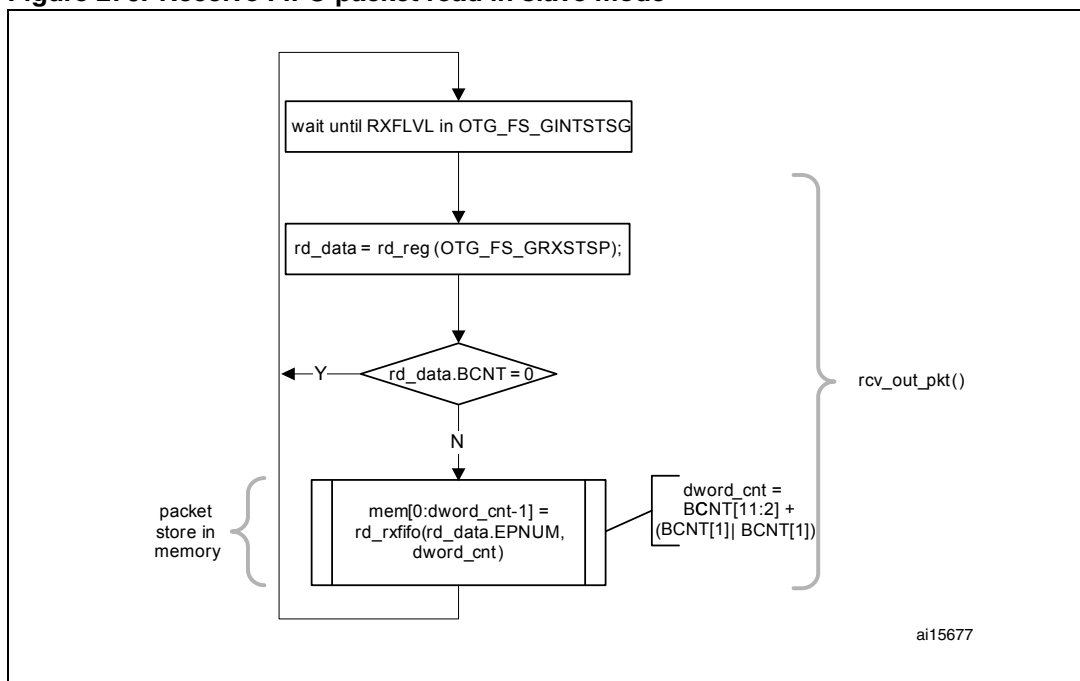
Figure 276. Receive FIFO packet read in slave mode
