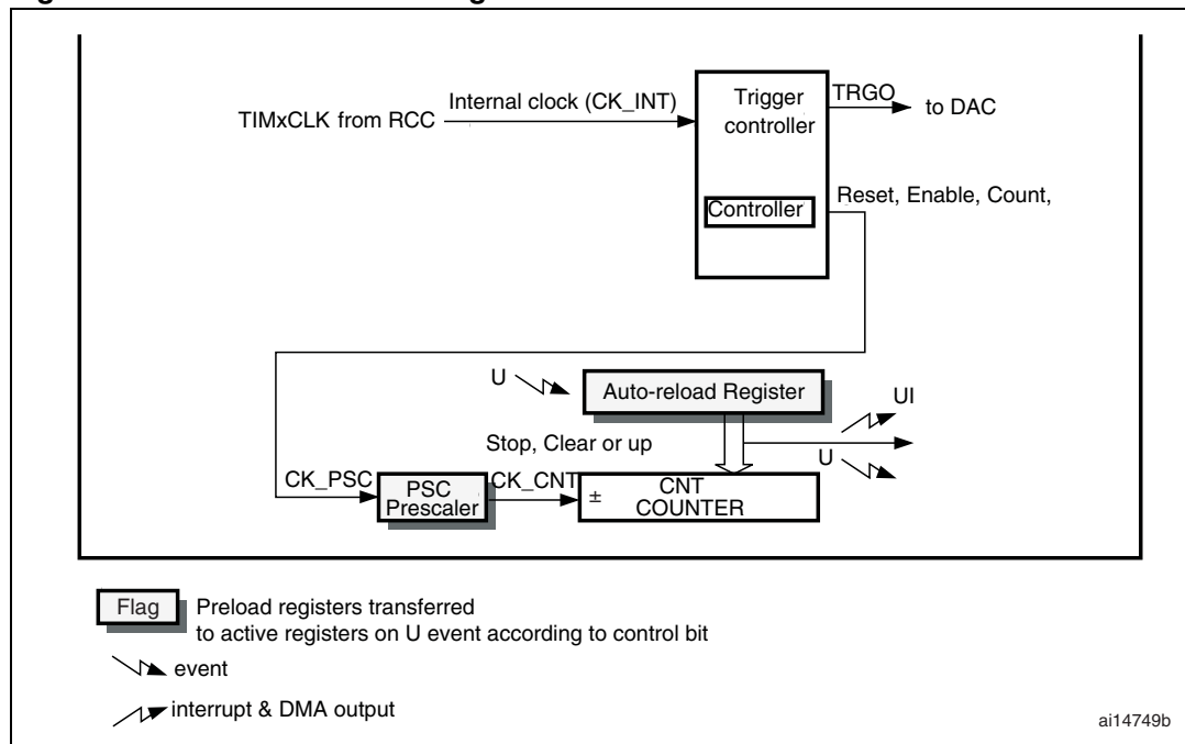
Figure 145. Basic timer block diagram
