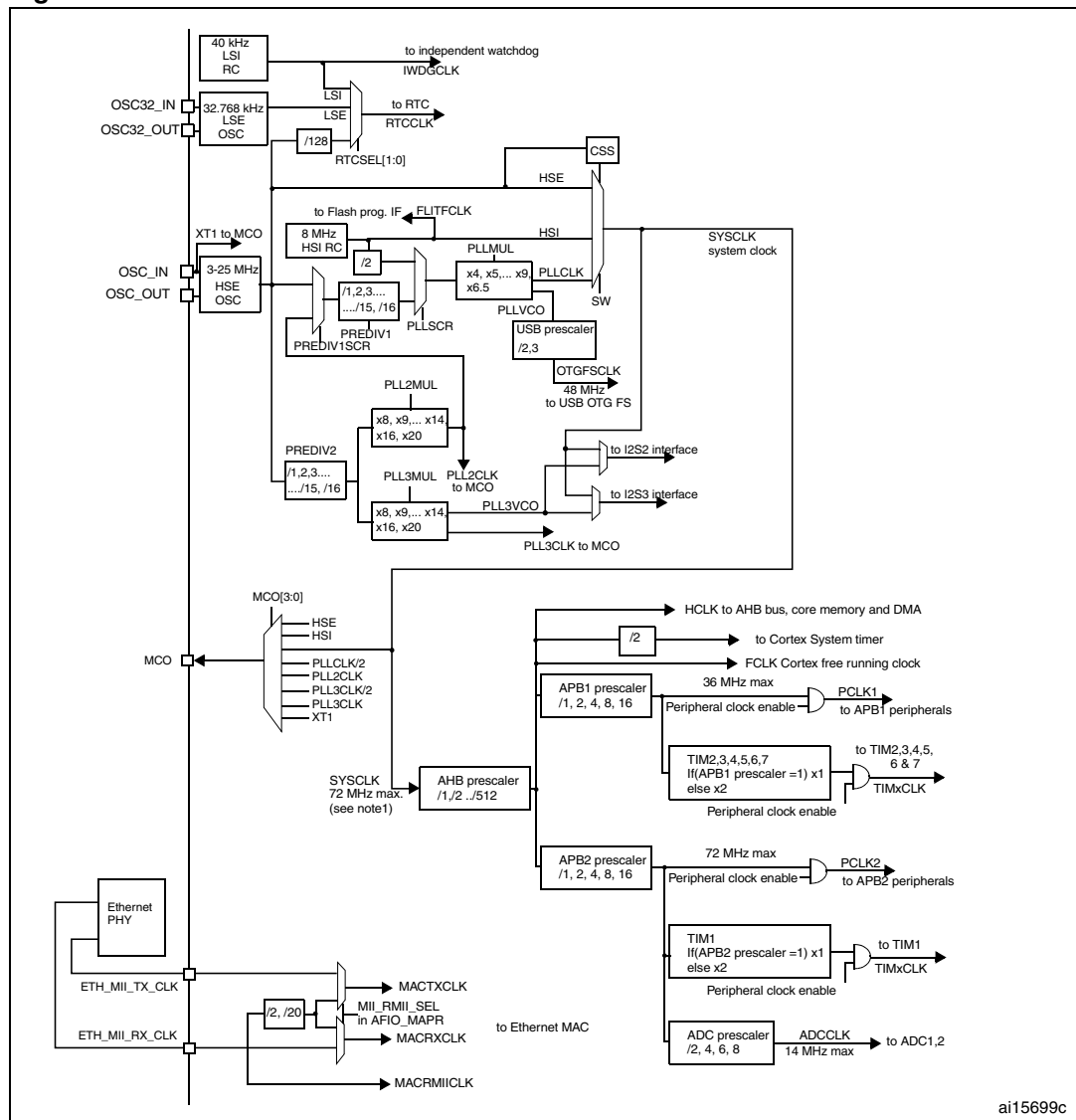
Figure 11. Clock tree
