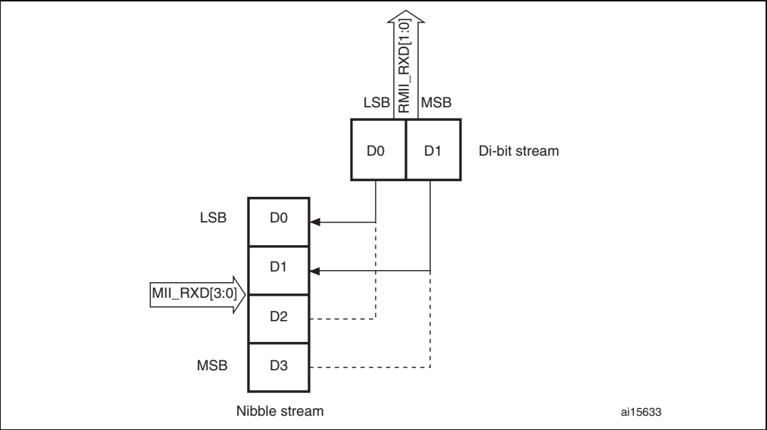
Figure 300. Receive bit order
