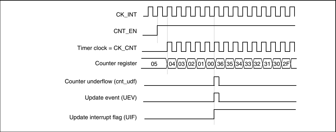
Figure 108. Counter timing diagram, internal clock divided by 1
