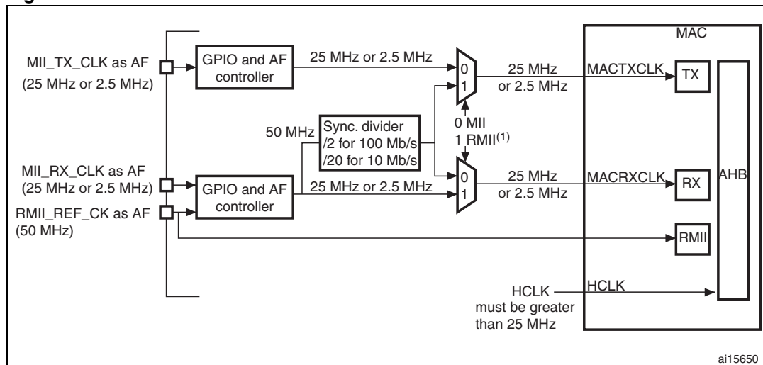
Figure 292. Clock scheme
