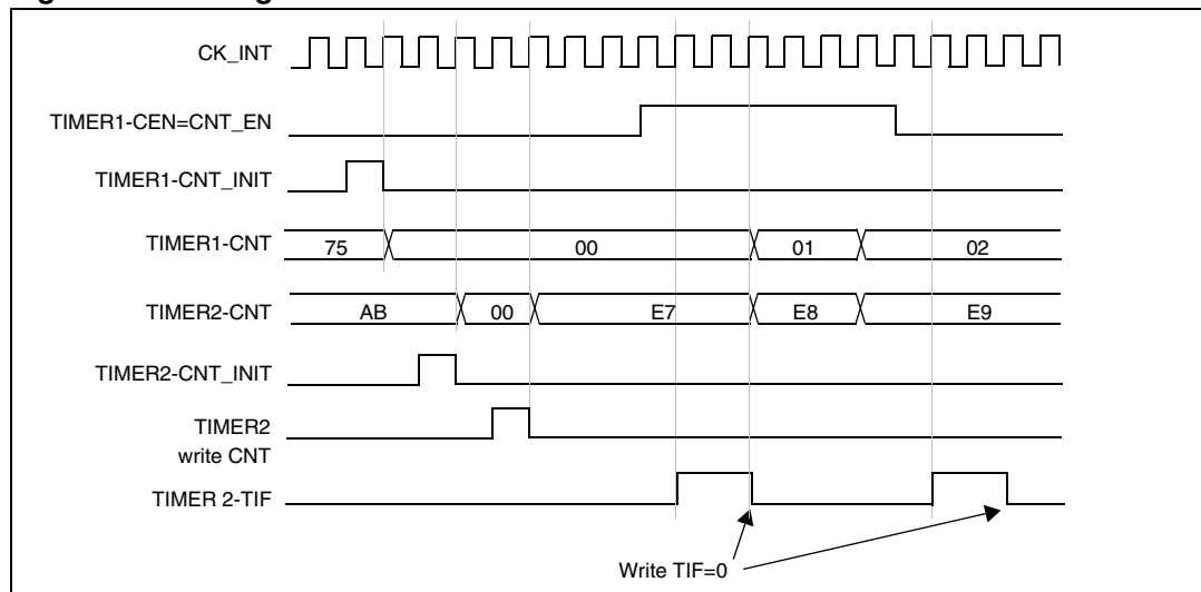
Figure 141. Gating timer 2 with Enable of timer 1
