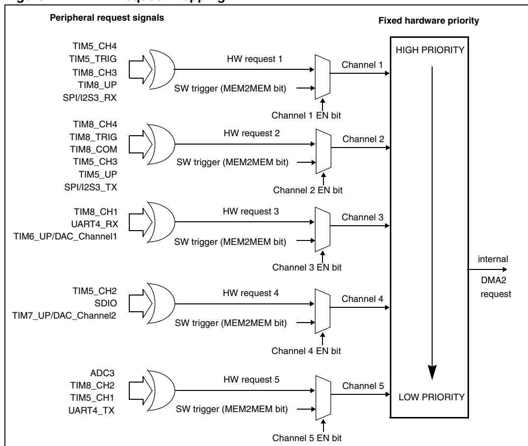
Figure 24. DMA2 request mapping
