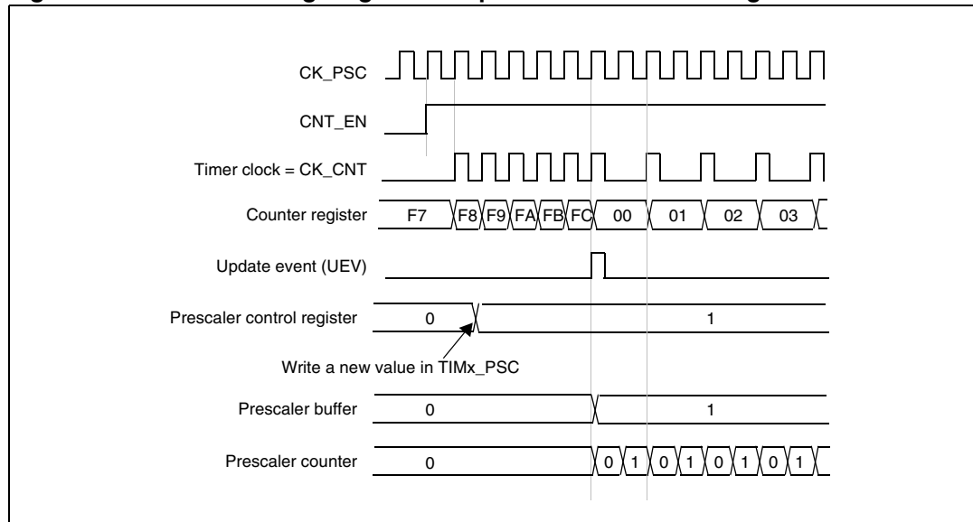
Figure 146. Counter timing diagram with prescaler division change from 1 to 2
