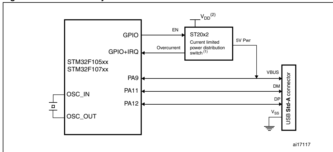
Figure 263. USB host only connection
