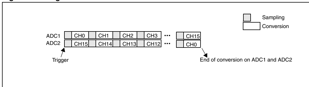
Figure 34. Regular simultaneous mode on 16 channels
