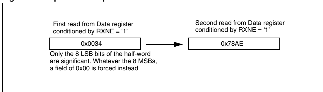
Figure 224. Operations required to receive 0x3478AE
