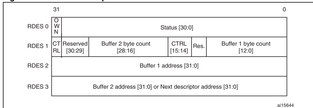
Figure 316. Rx DMA descriptor structure
