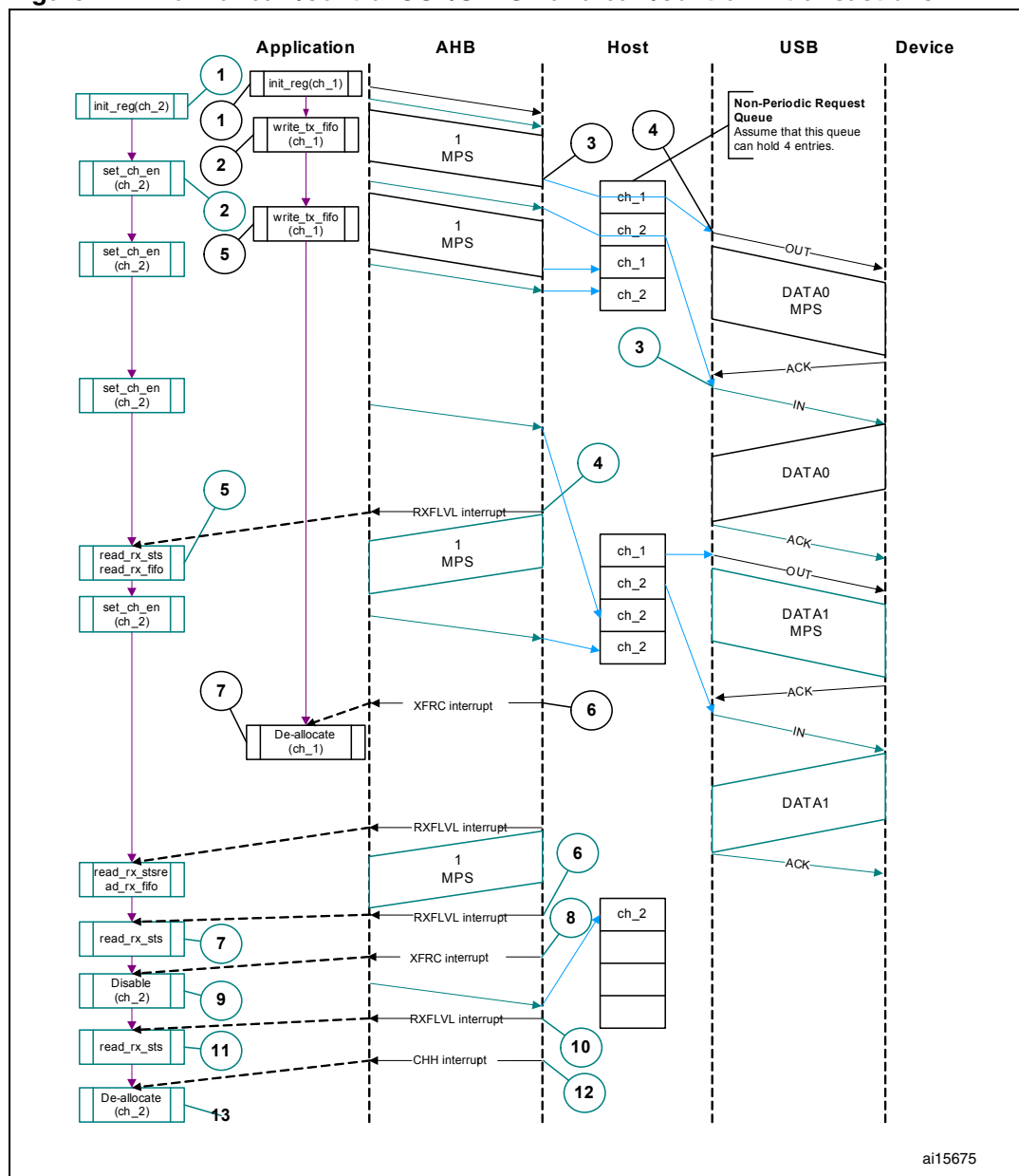
Figure 272. Normal bulk/control OUT/SETUP and bulk/control IN transactions
