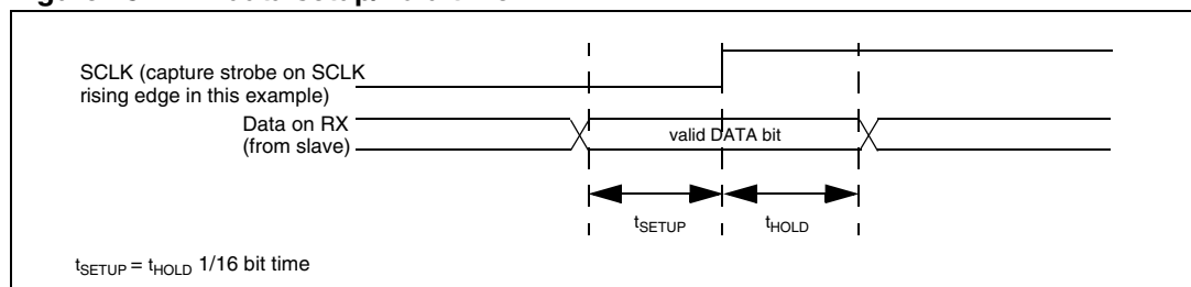
Figure 251. RX data setup/hold time
