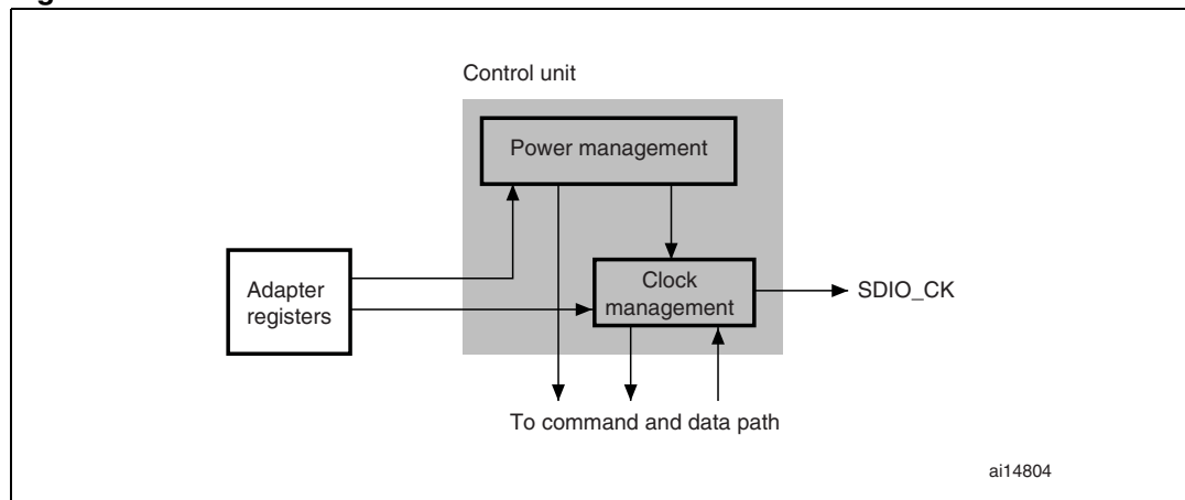
Figure 184. Control unit
