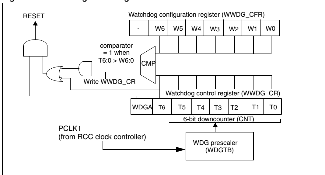
Figure 159. Watchdog block diagram
