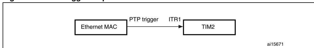
Figure 308. PTP trigger output to TIM2 ITR1 connection
