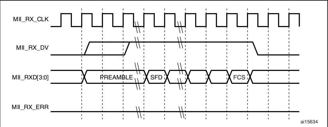
Figure 301. Reception with no error
