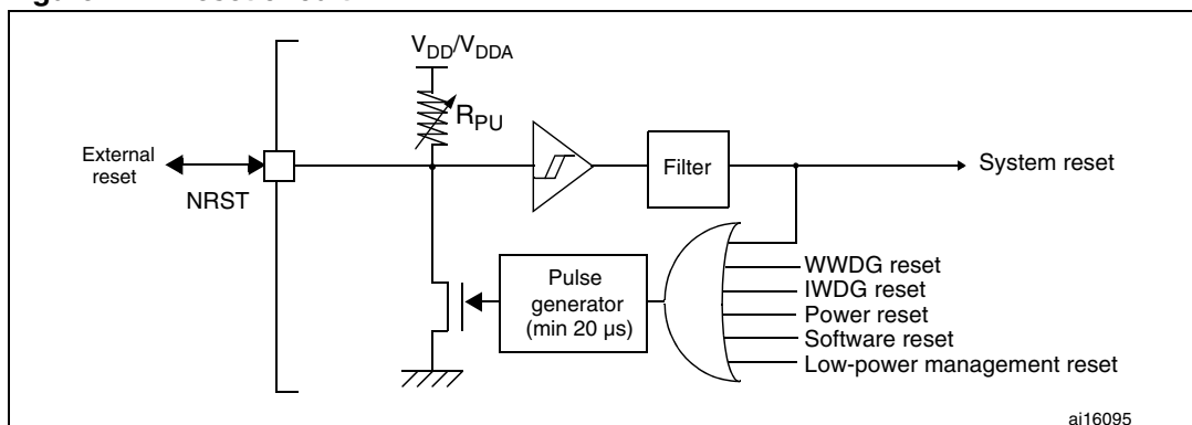
Figure 7. Reset circuit
