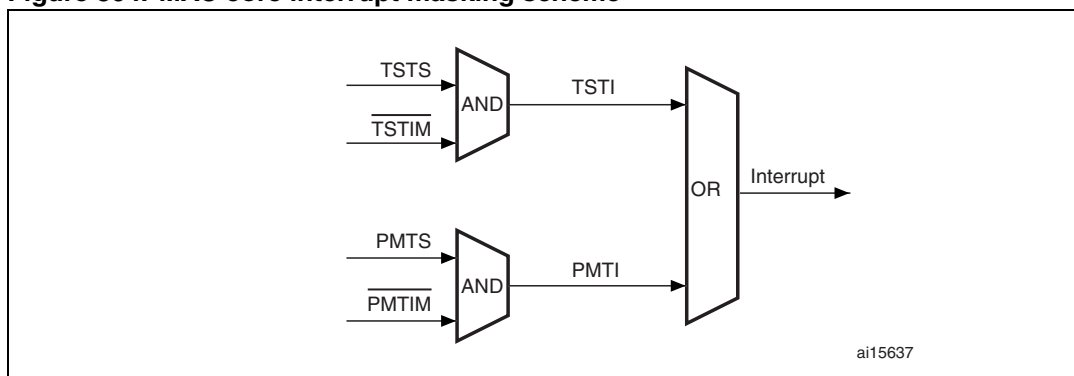
Figure 304. MAC core interrupt masking scheme
