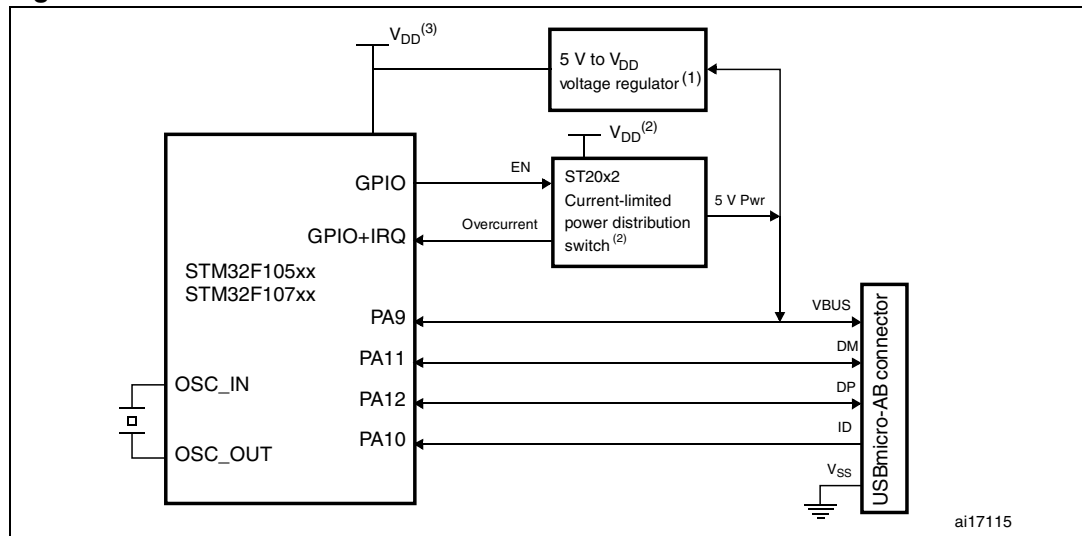
Figure 261. OTG A-B device connection
