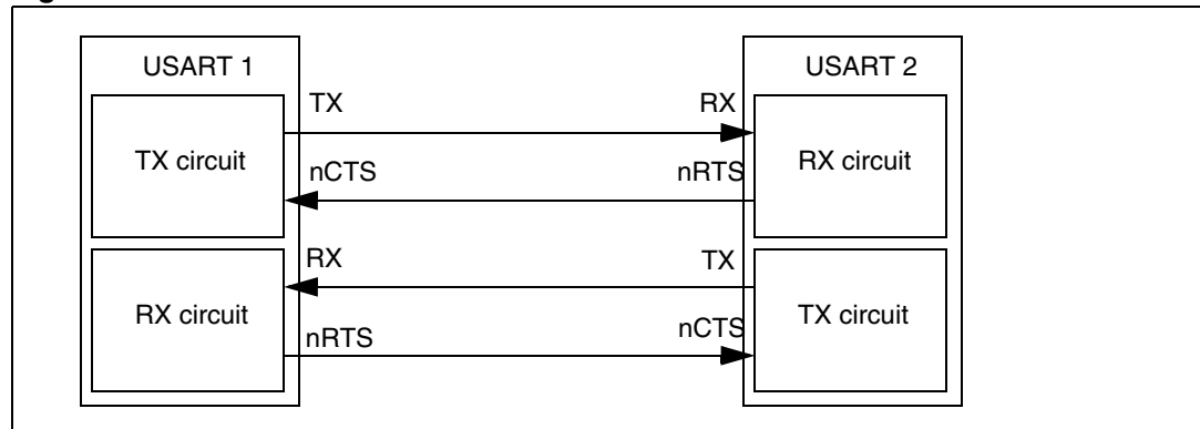
Figure 256. Hardware flow control between 2 USART
