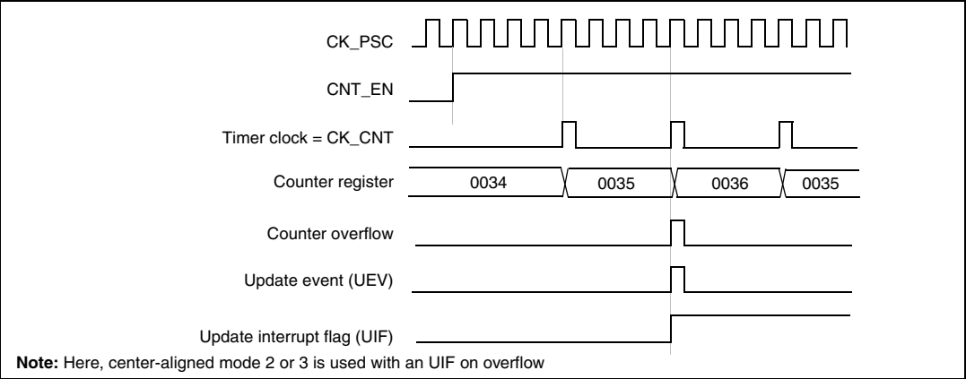
Figure 67. Counter timing diagram, internal clock divided by 4, TIMx_ARR=0x36
