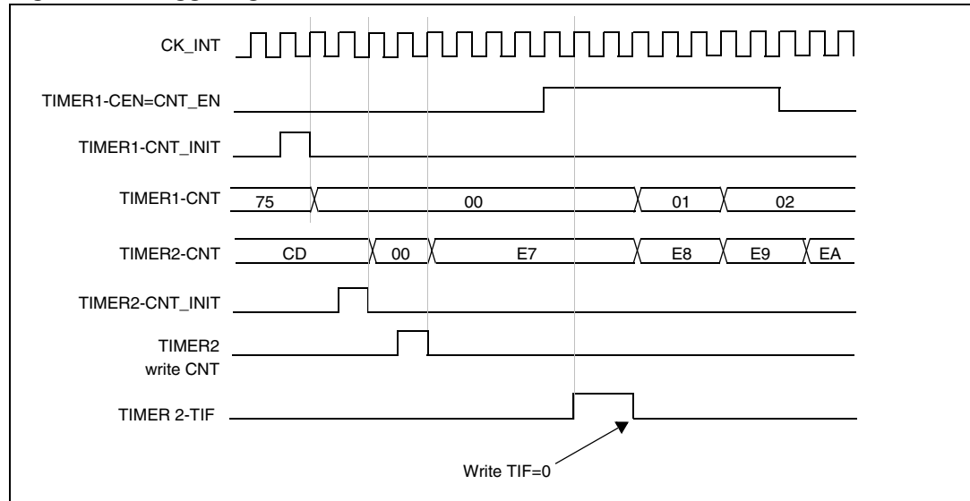
Figure 143. Triggering timer 2 with Enable of timer 1
