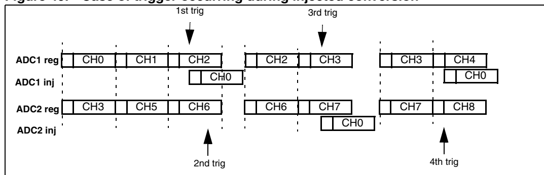
Figure 40. Case of trigger occurring during injected conversion
