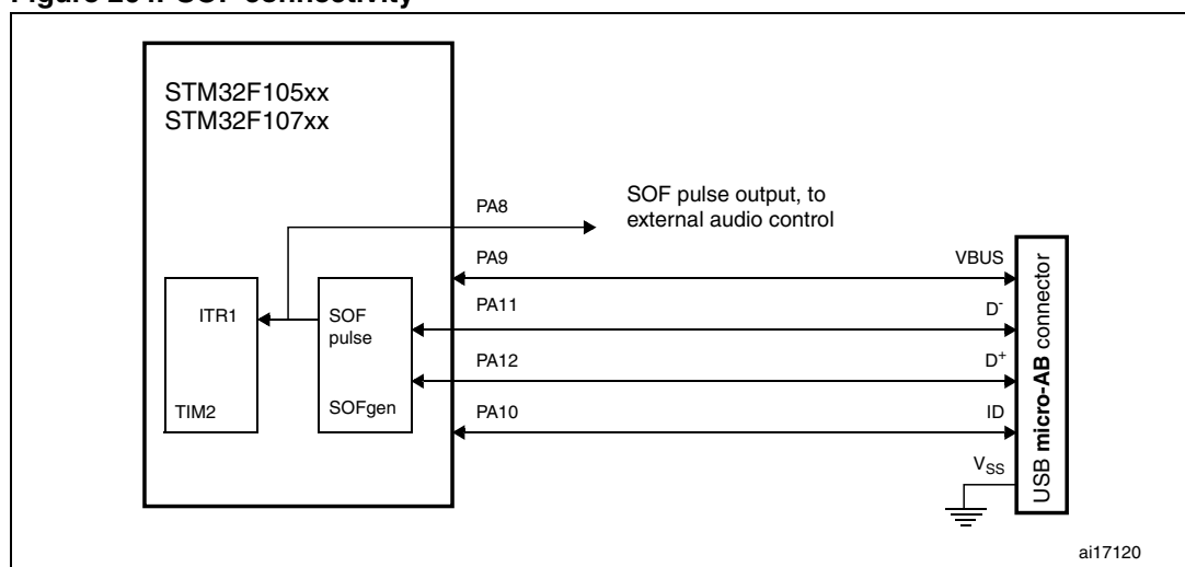
Figure 264. SOF connectivity
