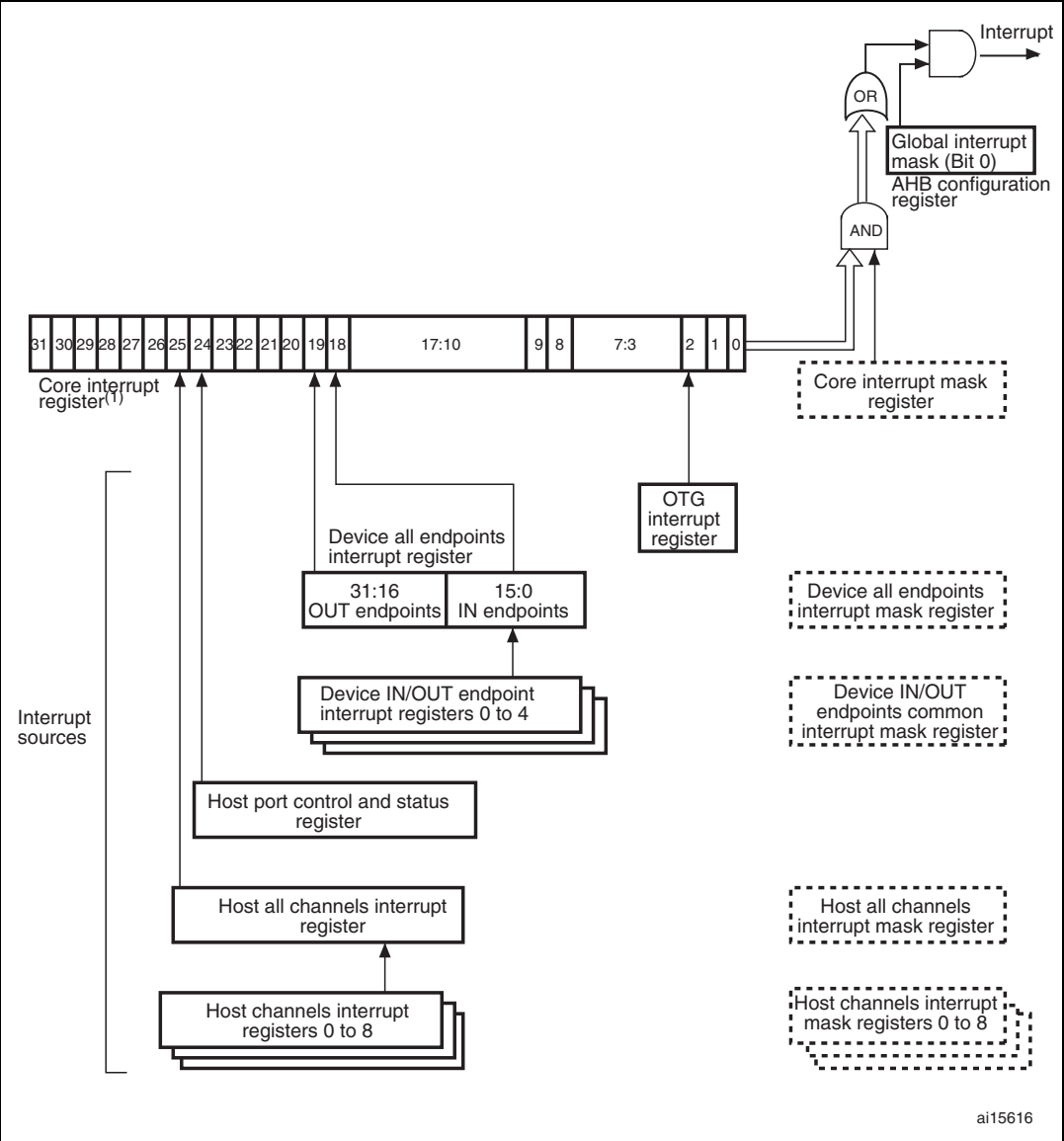
Figure 268. Interrupt hierarchy
