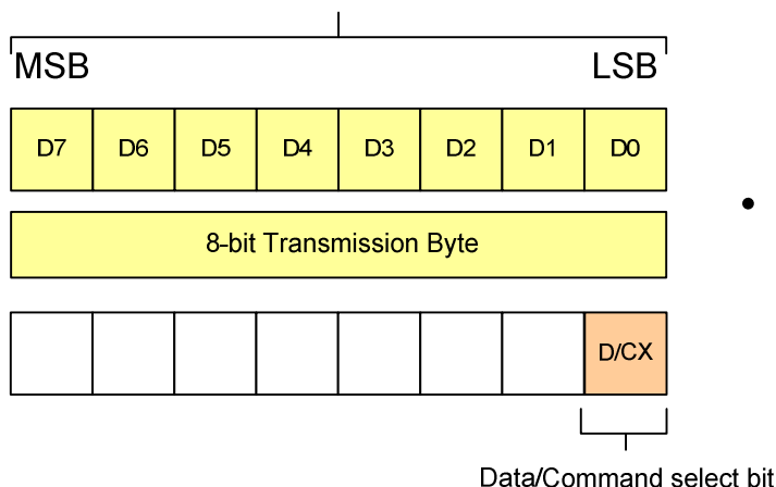
Figure 6: DBI Type C (Option 3) Data Format
