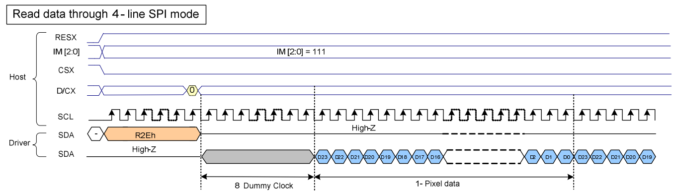
Figure 108: 4-Line SPI Mode Read Data
