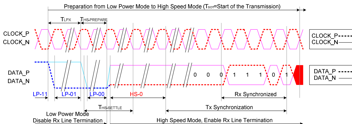
Figure 37: Entering High-Speed Data Transmission ( T_{SOT} of HSDT)
