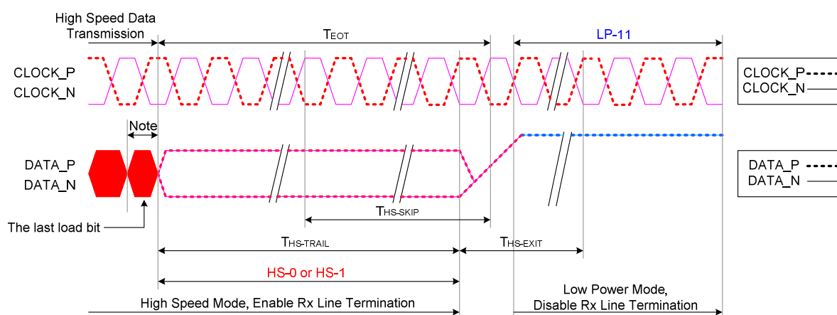
Figure 38: Leaving High-Speed Data Transmission
