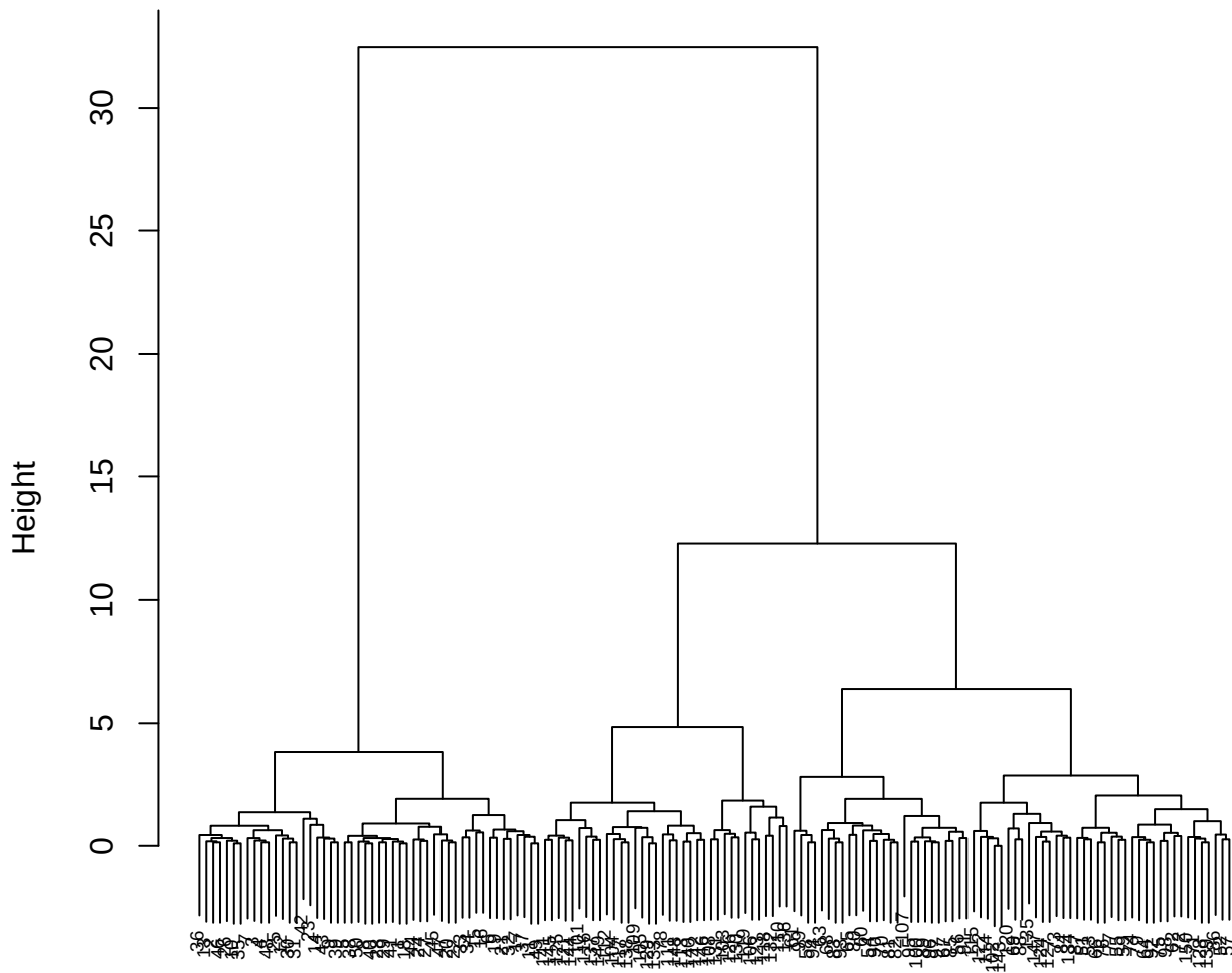
Hierarchical Clustering Dendrogram (Ward.D2)
