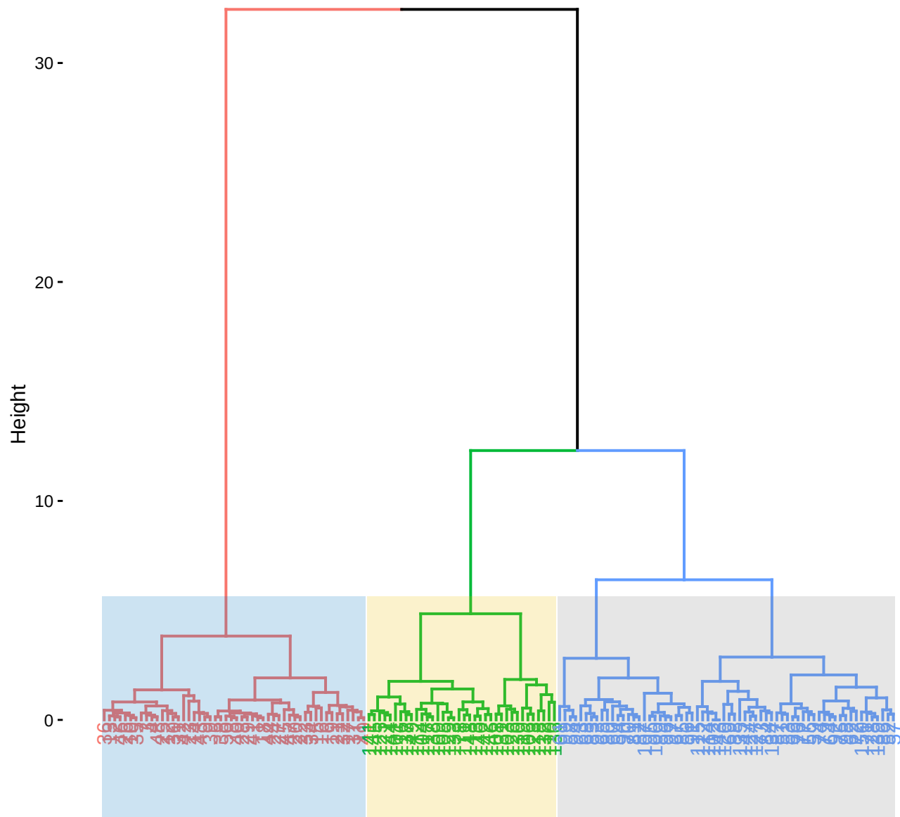
Dendrogram with Cluster Rectangles
