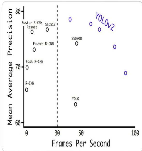
Fig.8.1. Mean average
