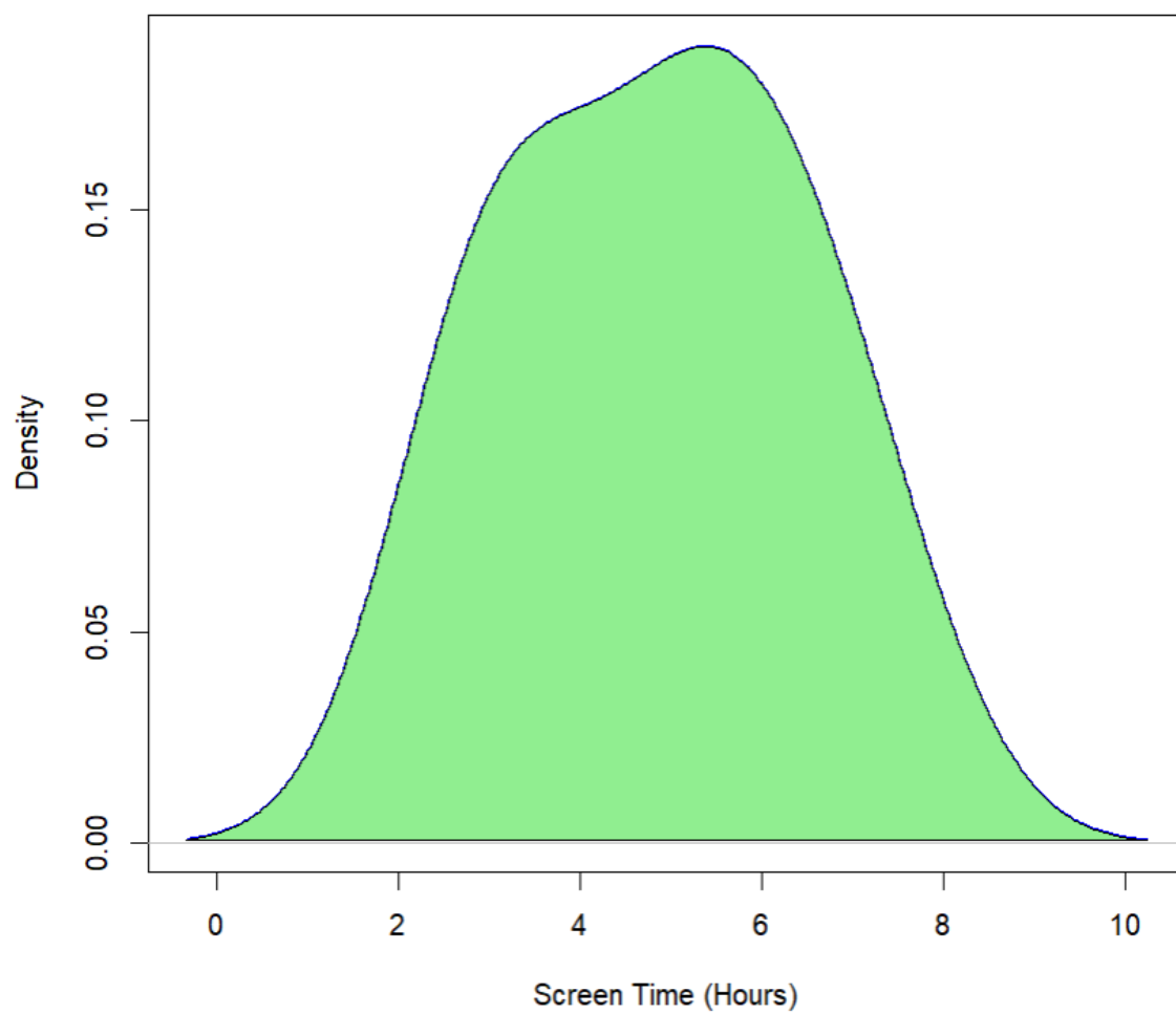
Density Plot of Screen Time
