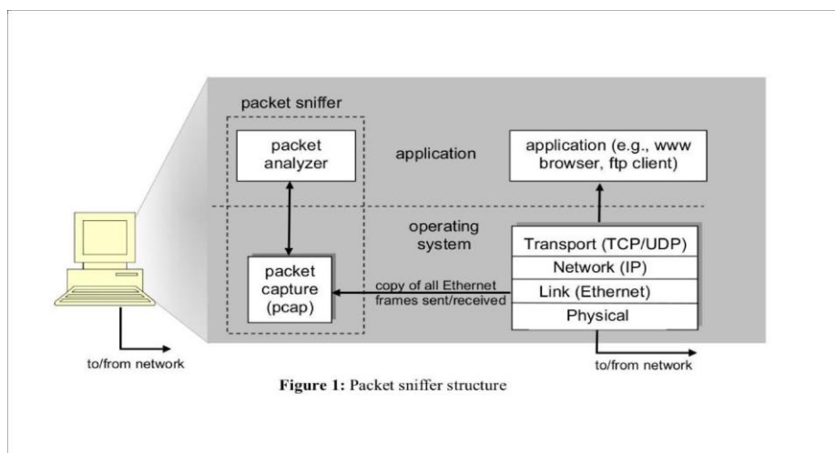
Fig. 1 — Packet sniffer structure: the packet capture (pcap) layer receives a copy of Ethernet frames sent/received by the protocol stack, and the packet analyser displays them
