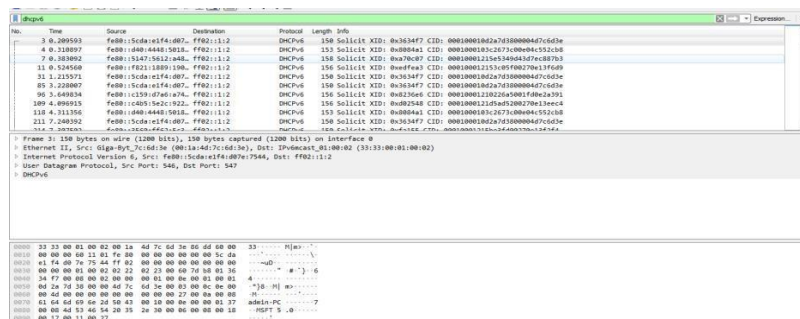
Fig. 5 — Filtered DHCPv6 packets showing Solicit messages
