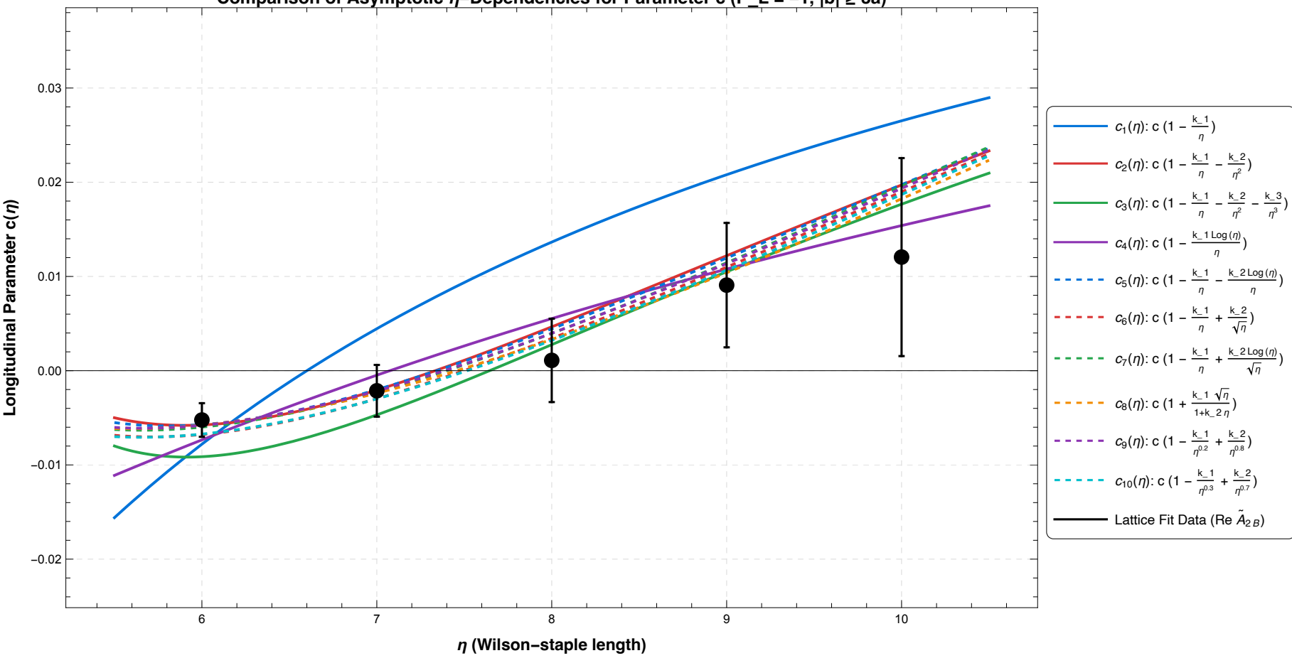
Comparison of Asymptotic \eta -Dependencies for Parameter c ( P_L = -1 , |b| \geq 3a )
